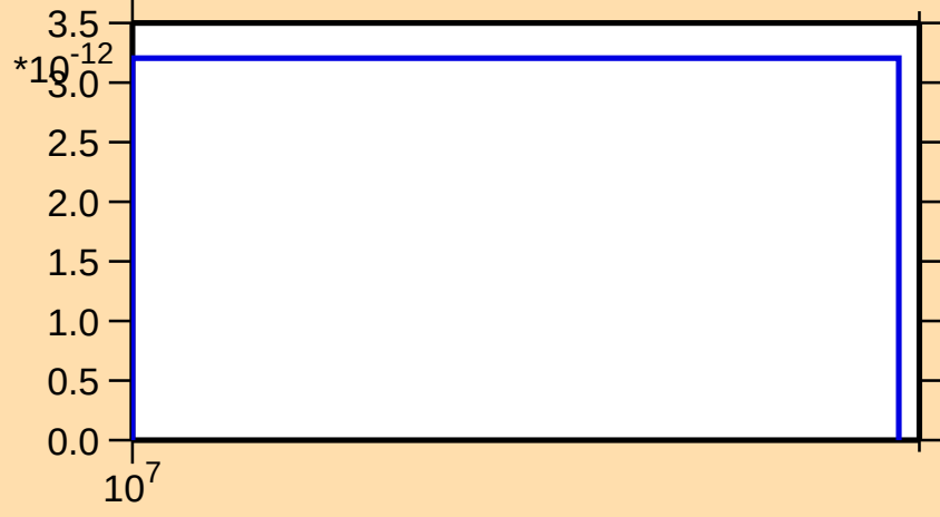
\sigma vs. E for ^{41}\text{Ar}(n,nt)
