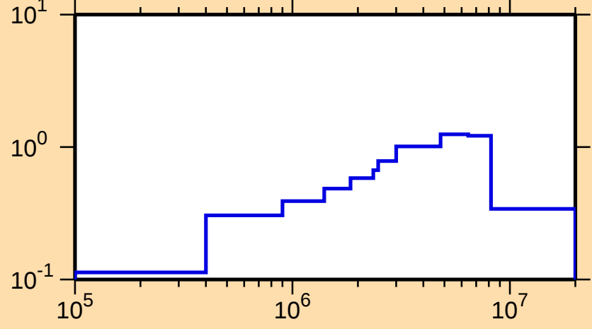
\sigma vs. E for ^{41}\text{Ar}(n,\text{inel.})
