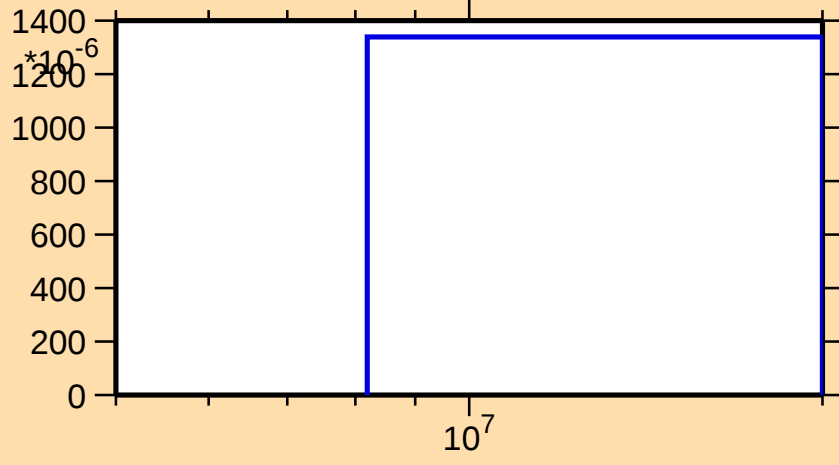
\sigma vs. E for ^{41}\text{Ar}(n,n\alpha)
