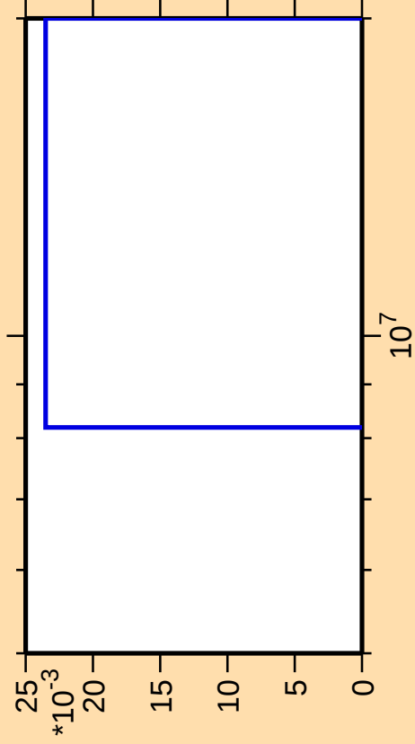
\Delta\sigma/\sigma vs. E for ^{41}\text{Ar}(n,\text{He}3)
