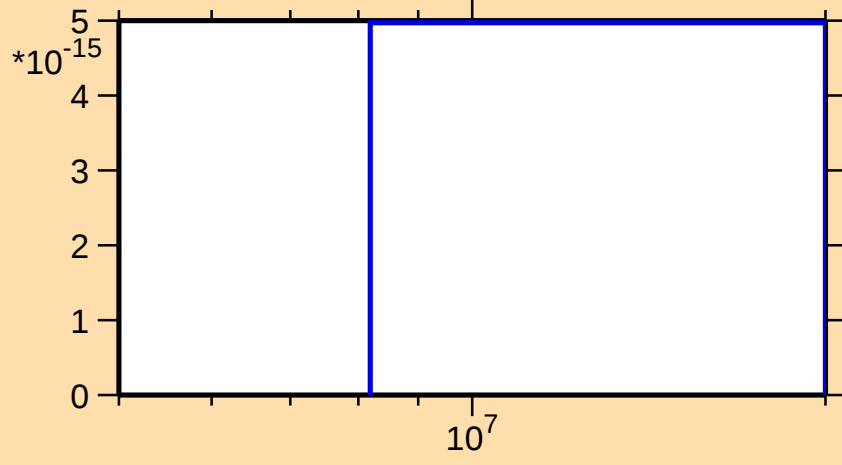
\sigma vs. E for ^{41}\text{Ar}(n,\text{He}3)
