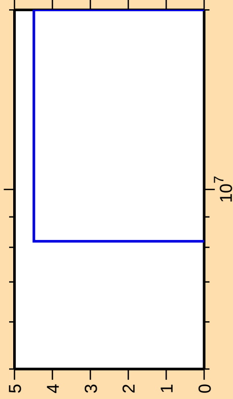
\Delta\sigma/\sigma vs. E for ^{41}\text{Ar}(n,nt)
