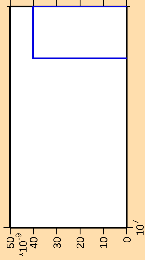
\Delta\sigma/\sigma vs. E for ^{42}\text{Ar}(n,\text{He}3)
