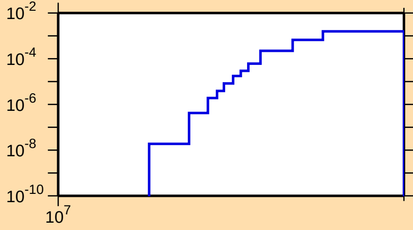
\sigma vs. E for ^{42}\text{Ar}(n,n\alpha)
