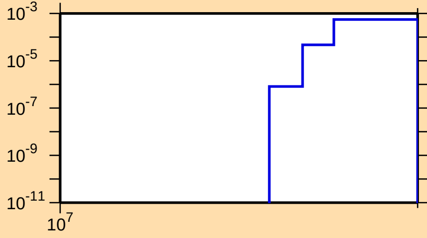
\sigma vs. E for ^{42}\text{Ar}(n,np)
