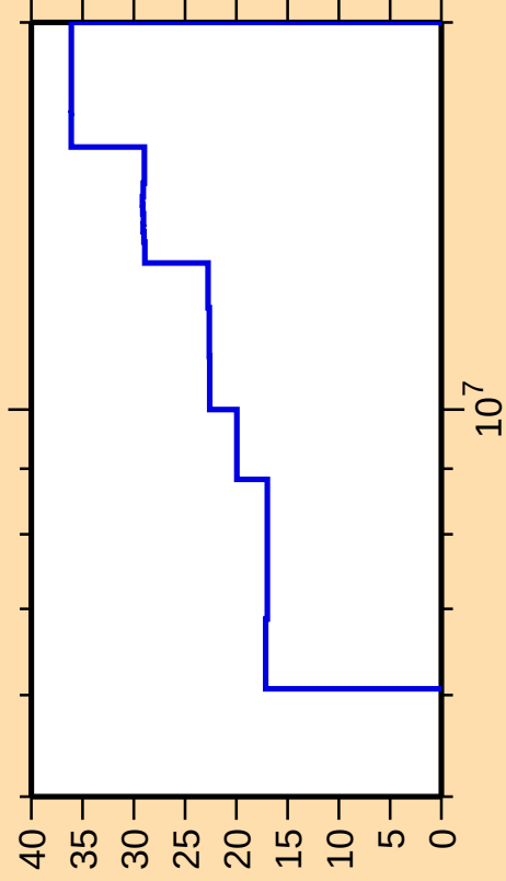
\Delta\sigma/\sigma vs. E for ^{42}\text{Ar}(n,\text{ncont.})
