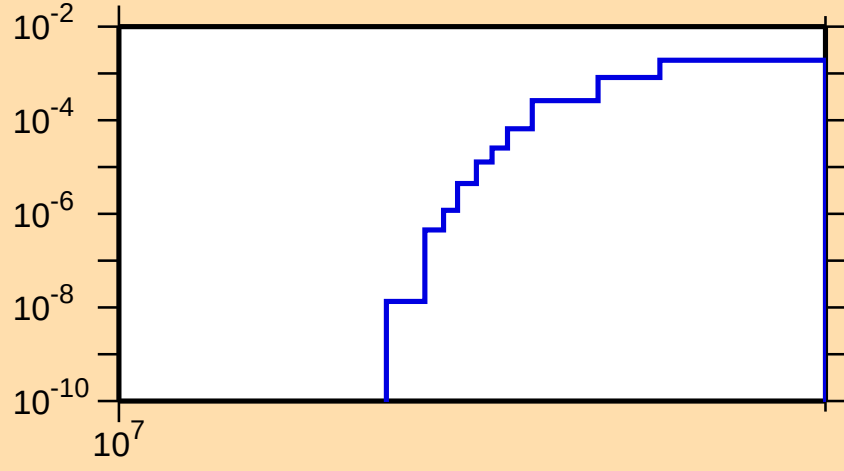
\sigma vs. E for ^{42}\text{Ar}(n,d)
