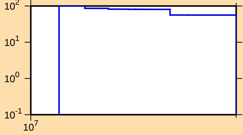
\Delta\sigma/\sigma vs. E for ^{71}\text{As}(n,2n)
