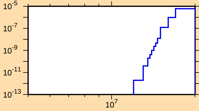
\sigma vs. E for ^{71}\text{As}(\text{mt117})
