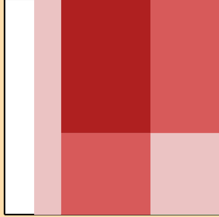
\Delta\sigma/\sigma vs. E for ^{71}\text{As}(n,2n)
