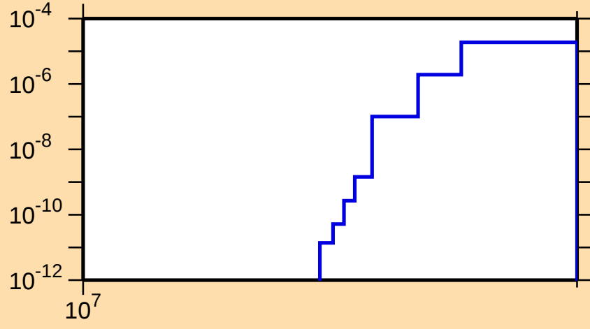
\sigma vs. E for ^{71}\text{As}(n,\text{pd})
