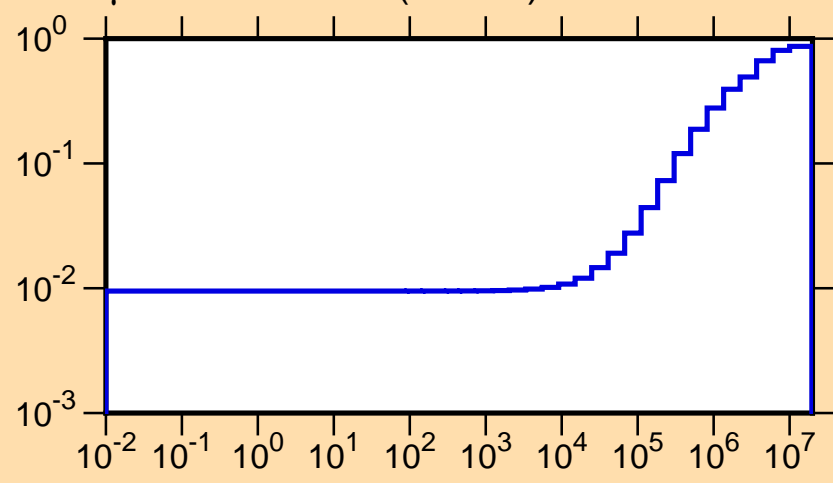
\mu vs. E for ^{71}\text{As}(\text{mt251})
