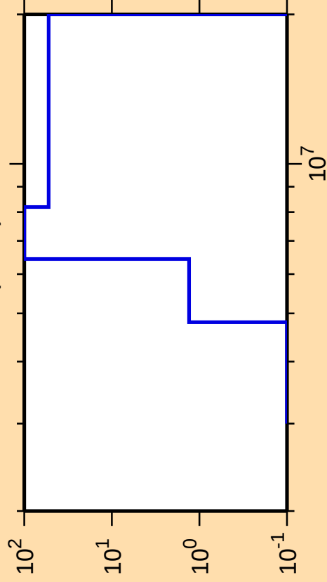
\Delta\sigma/\sigma vs. E for ^{71}\text{As}(n,n\alpha)
