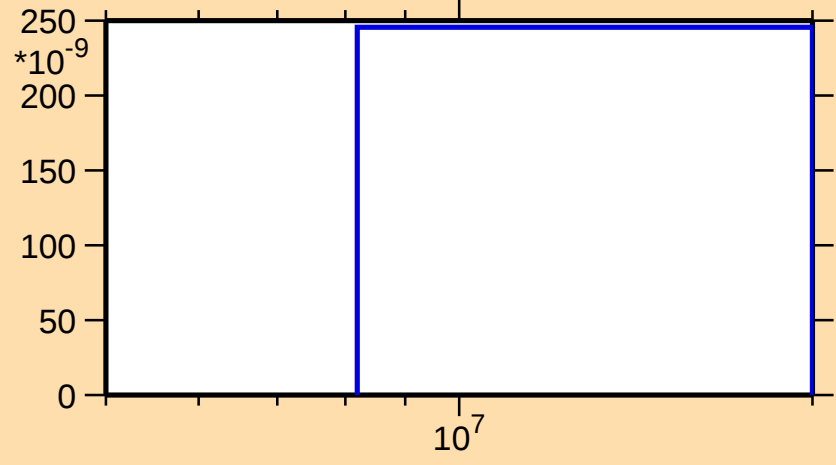
\sigma vs. E for ^{71}\text{As}(\text{mt } 45)
