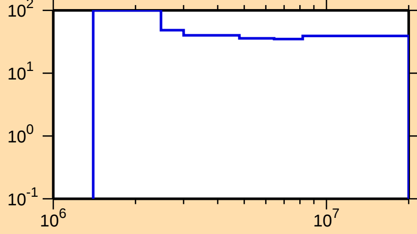
\Delta\sigma/\sigma vs. E for ^{71}\text{As}(n,ncont.)
