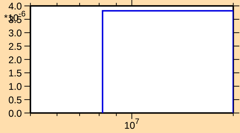
\sigma vs. E for ^{71}\text{As}(n,\text{He3})
