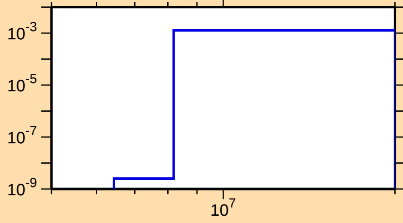
\sigma vs. E for ^{71}\text{As}(n,p\alpha)
