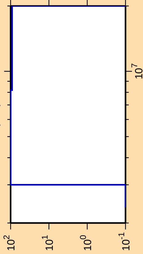
\Delta\sigma/\sigma vs. E for ^{71}\text{As}(n,d)
