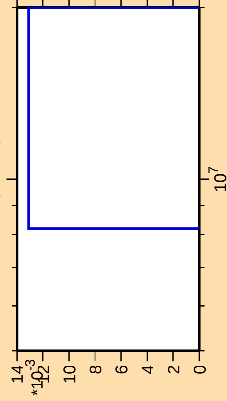
\Delta\sigma/\sigma vs. E for ^{71}\text{As}(\text{mt } 34)
