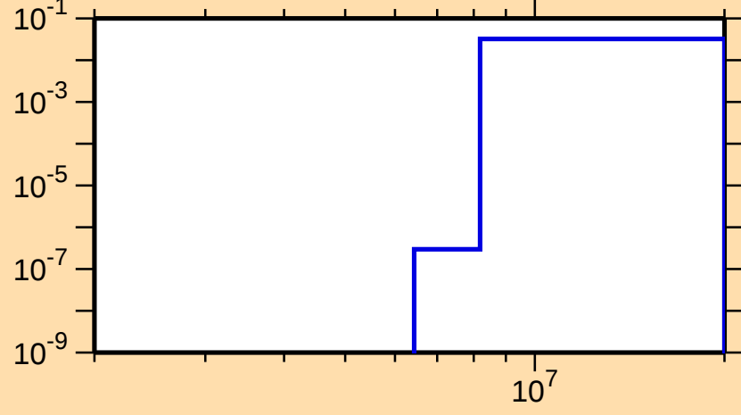
\sigma vs. E for ^{71}\text{As}(n,n\alpha)
