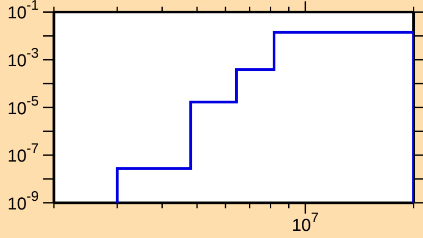
\sigma vs. E for ^{71}\text{As}(n,d)
