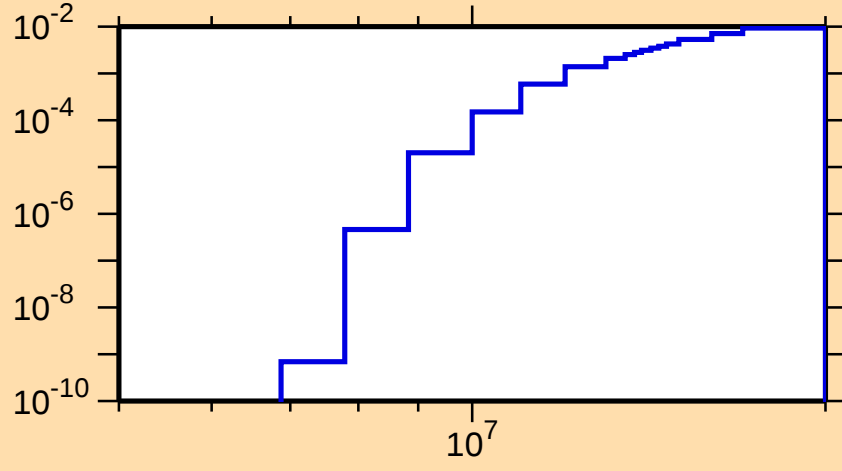
\sigma vs. E for ^{77}\text{As}(n,d)
