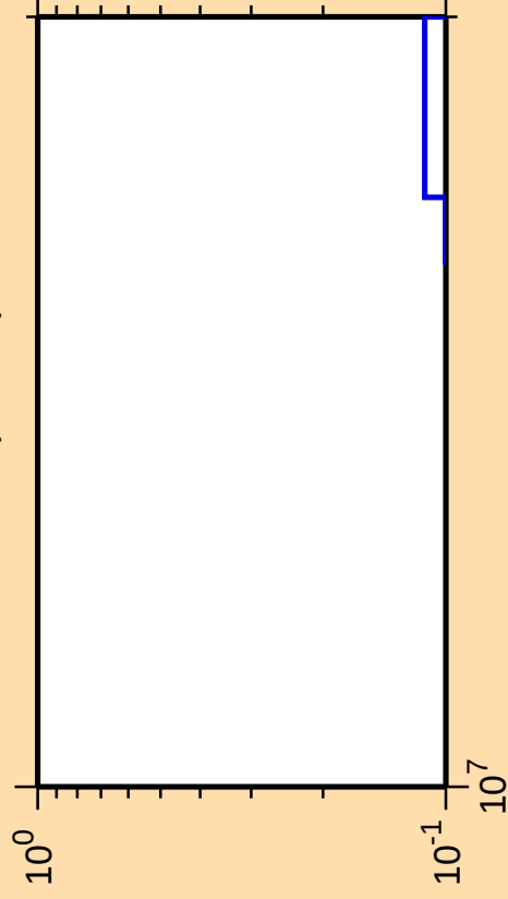
\Delta\sigma/\sigma vs. E for ^{77}\text{As}(n,2n\alpha)
