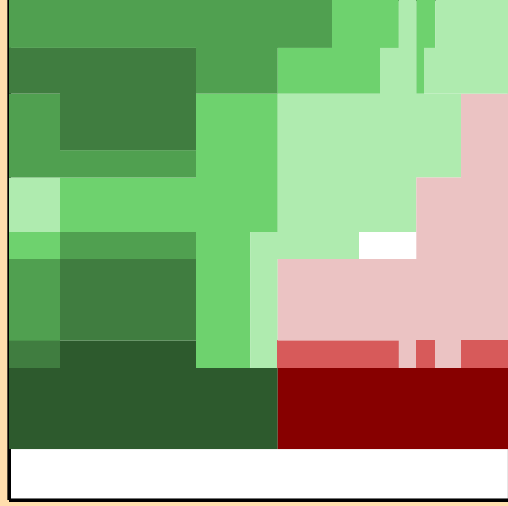
\Delta\sigma/\sigma vs. E for ^{77}\text{As}(n,n_1)
