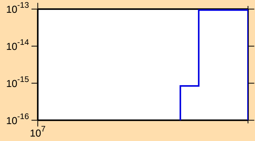
\sigma vs. E for ^{77}\text{As}(n,2n\alpha)
