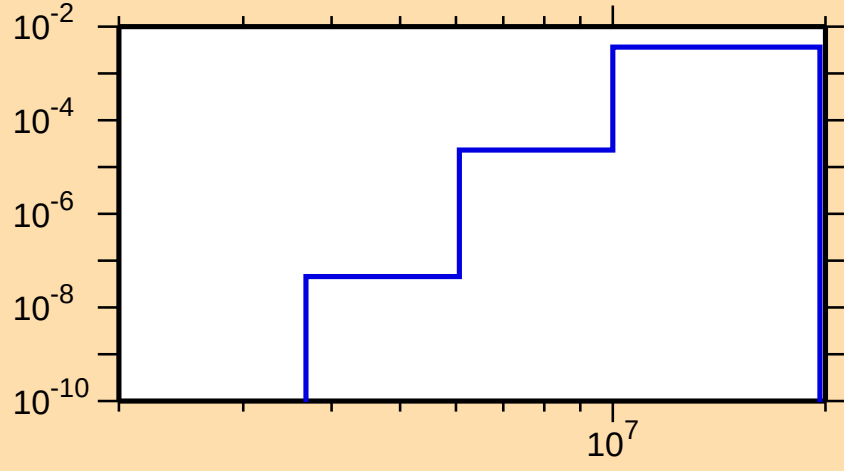
\sigma vs. E for ^{77}\text{As}(n,\alpha)
