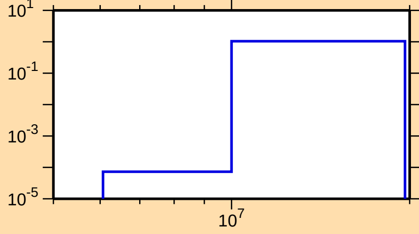
\sigma vs. E for ^{77}\text{As}(n,2n)
