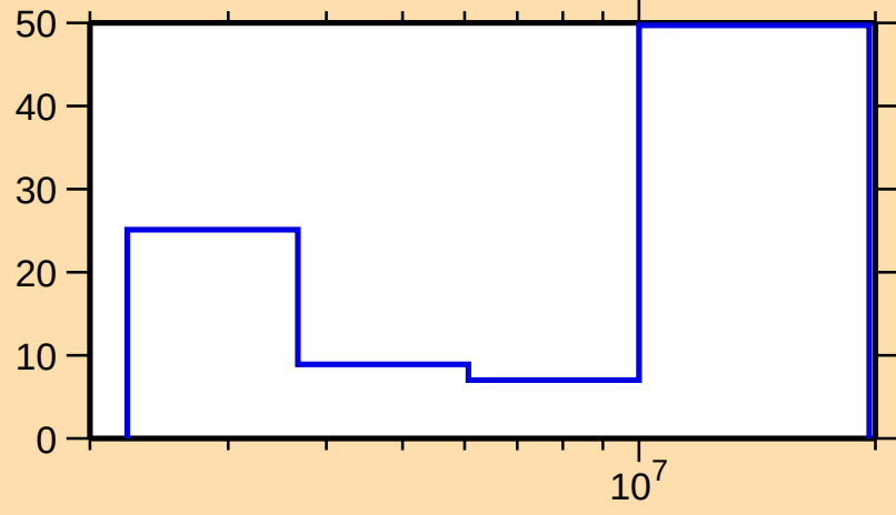
\Delta\sigma/\sigma vs. E for ^{77}\text{As}(n,n\text{cont.})
