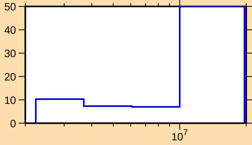
\Delta\sigma/\sigma vs. E for ^{77}\text{As}(n,\text{inel.})
