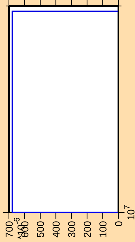
\Delta\sigma/\sigma vs. E for ^{77}\text{As}(n,2n\alpha)
