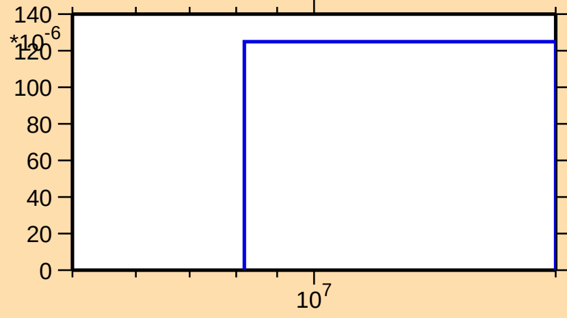
\sigma vs. E for ^{77}\text{As}(n,\alpha)
