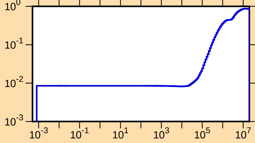
\mu vs. E for ^{79}\text{As}(\text{mt251})
