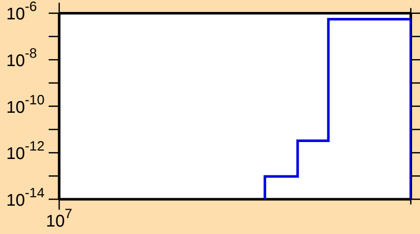
\sigma vs. E for ^{79}\text{As}(n,\text{nd})
