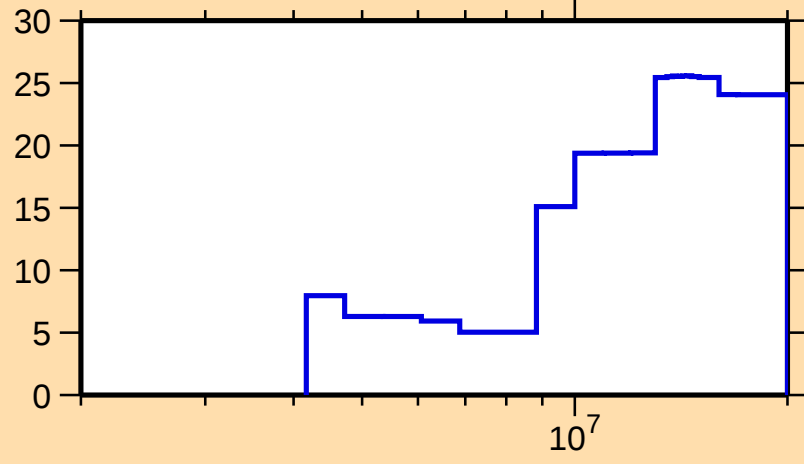
\Delta\sigma/\sigma vs. E for ^{79}\text{As}(n,n\text{cont.})
