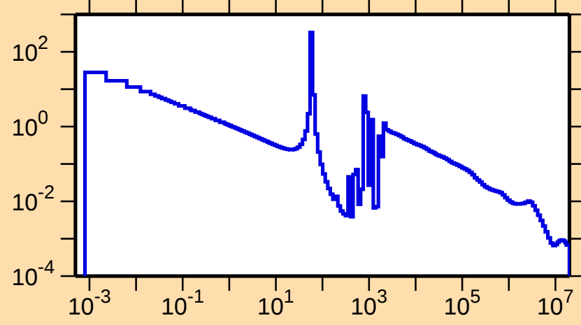
\sigma vs. E for ^{79}\text{As}(n,\gamma)
