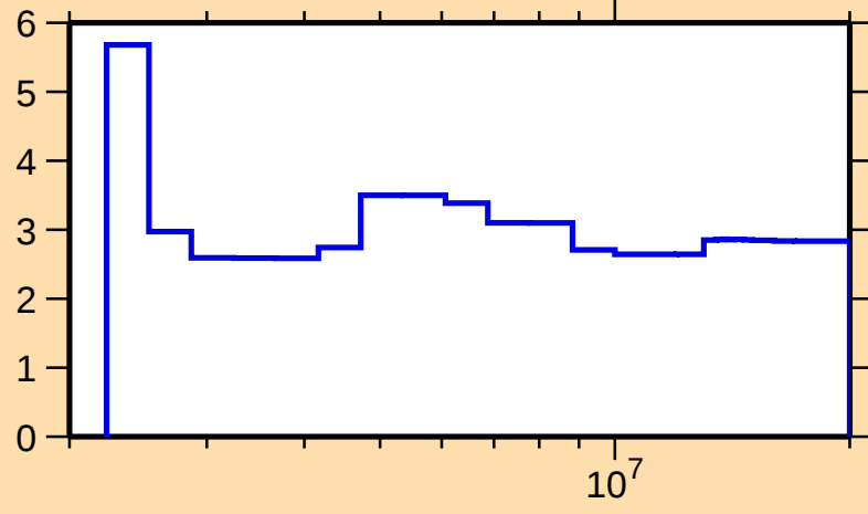
\Delta\sigma/\sigma vs. E for ^{79}\text{As}(n,\text{nonel.})
