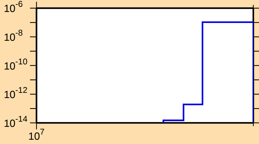
\sigma vs. E for ^{79}\text{As}(n,nt)
