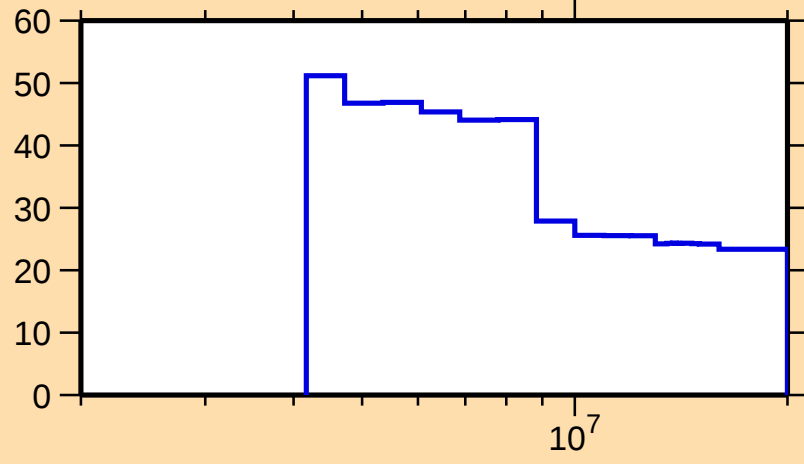
\Delta\sigma/\sigma vs. E for ^{79}\text{As}(n,\gamma)
