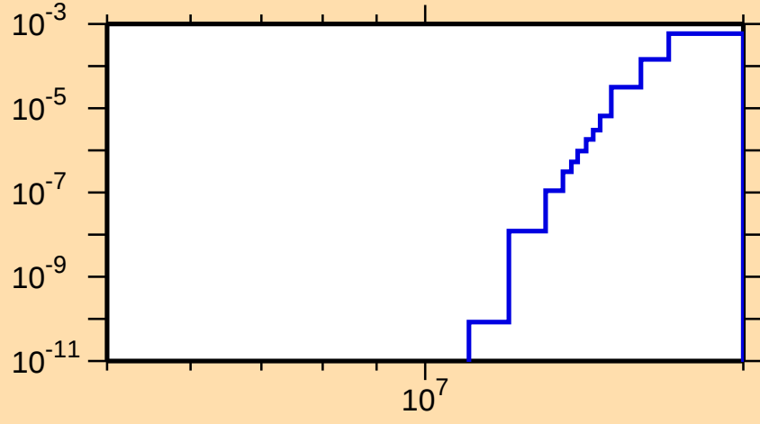
\sigma vs. E for ^{79}\text{As}(n,\alpha)
