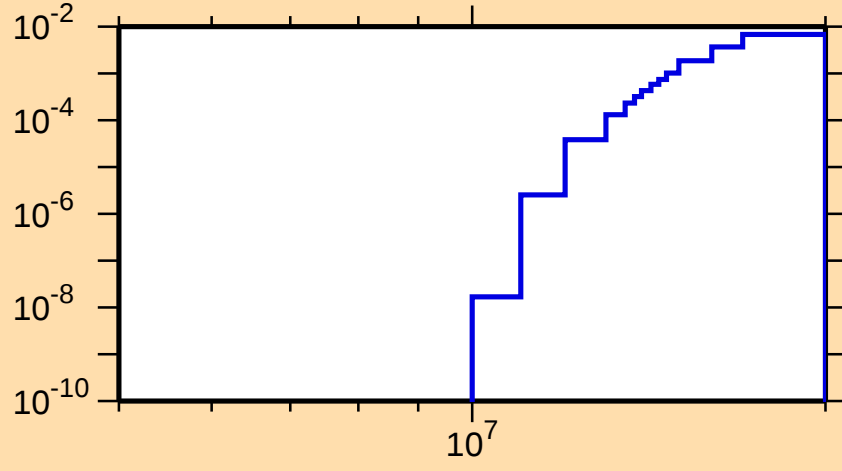
\sigma vs. E for ^{79}\text{As}(n,np)
