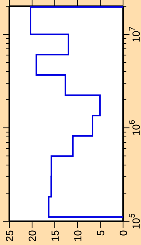
\Delta\sigma/\sigma vs. E for ^{79}\text{As}(n,n_2)
