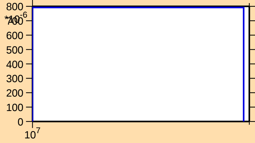
\sigma vs. E for ^{79}\text{As}(n,3n)
