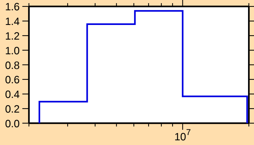
\sigma vs. E for ^{79}\text{As}(n,n\text{cont.})
