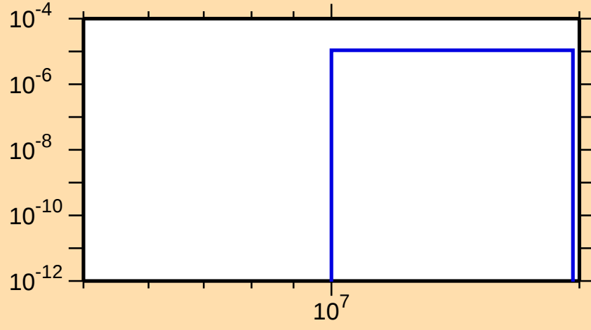
\sigma vs. E for ^{79}\text{As}(n,t)
