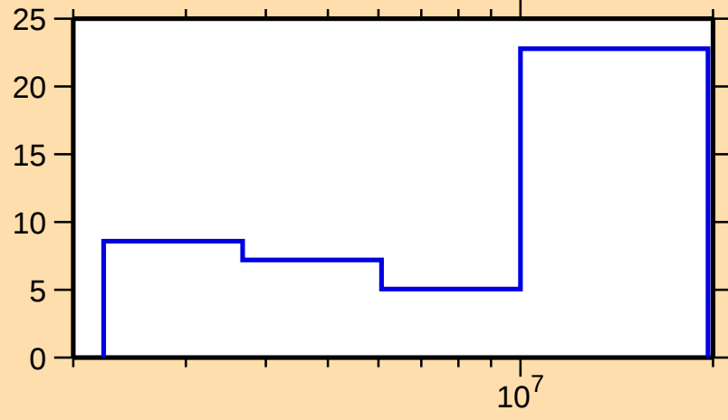
\Delta\sigma/\sigma vs. E for ^{79}\text{As}(n,ncont.)
