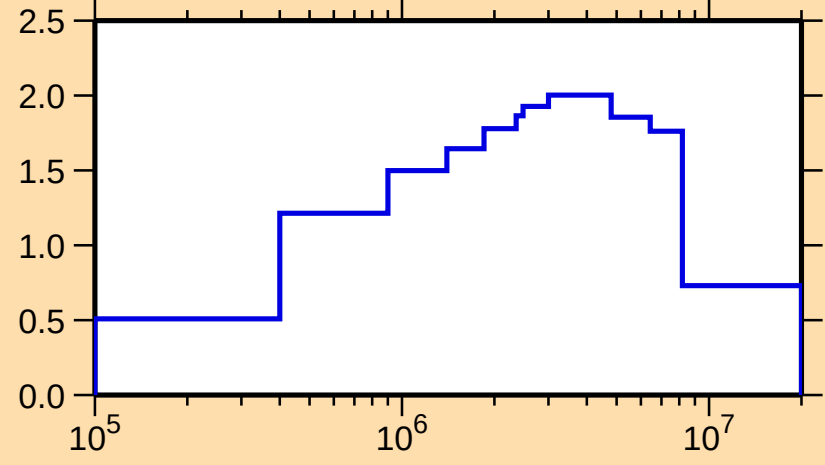
\sigma vs. E for ^{79}\text{As}(n,\text{inel.})
