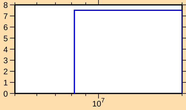
\Delta\sigma/\sigma vs. E for ^{79}\text{As}(n,2n)
