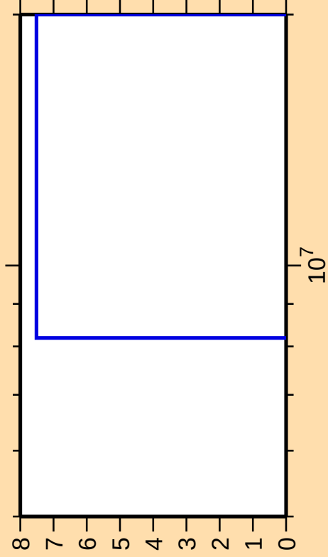
\Delta\sigma/\sigma vs. E for ^{79}\text{As}(n,2n)
