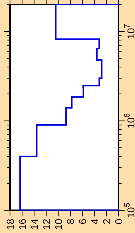
\Delta\sigma/\sigma vs. E for ^{79}\text{As}(\text{n,inel.})
