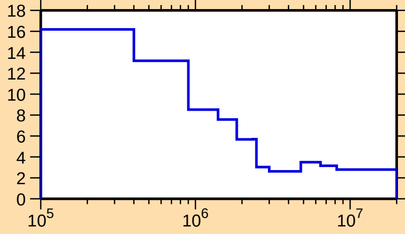
\Delta\sigma/\sigma vs. E for ^{79}\text{As}(\text{n,nonel.})
