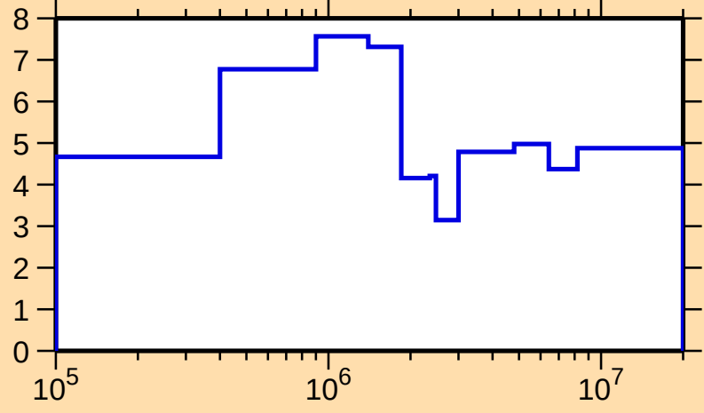
\Delta\sigma/\sigma vs. E for ^{79}\text{As}(\text{n,el.})
