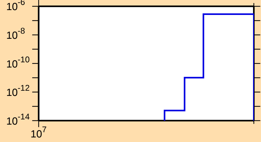
\sigma vs. E for ^{80}\text{As}(n,2np)
