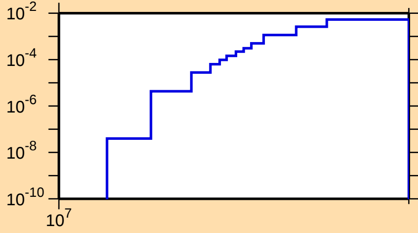
\sigma vs. E for ^{80}\text{As}(n,np)
