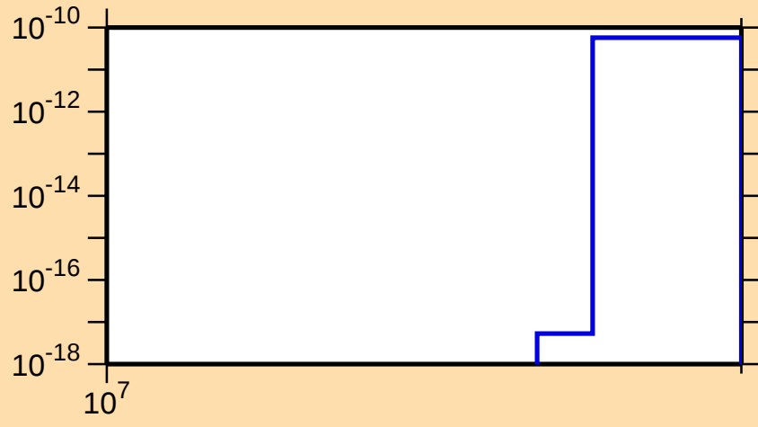
\sigma vs. E for ^{80}\text{As}(n,2n\alpha)
