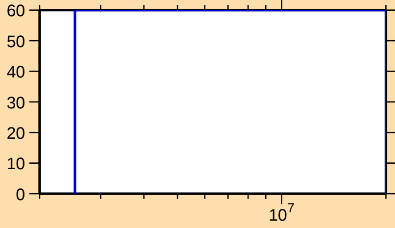
\Delta\sigma/\sigma vs. E for ^{80}\text{As}(n,p)
