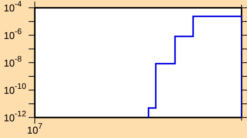
\sigma vs. E for ^{80}\text{As}(n,\text{nd})
