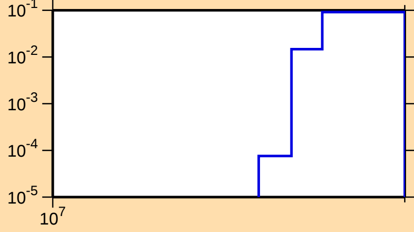
\sigma vs. E for ^{80}\text{As}(n,3n)
