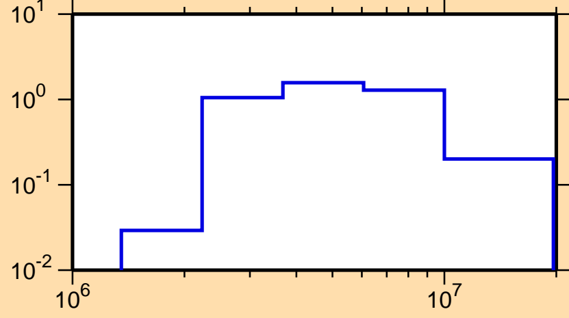
\sigma vs. E for ^{80}\text{As}(n,n\text{cont.})
