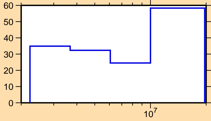
\Delta\sigma/\sigma vs. E for ^{80}\text{As}(n,ncont.)
