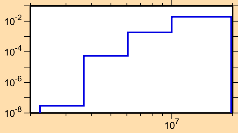
\sigma vs. E for ^{80}\text{As}(n,p)
