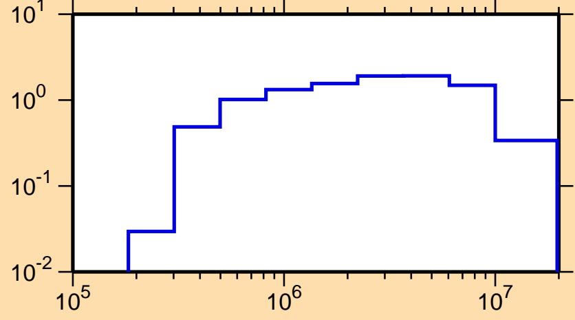
\sigma vs. E for ^{80}\text{As}(n,\text{inel.})
