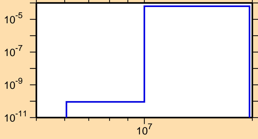
\sigma vs. E for ^{80}\text{As}(n,t)
