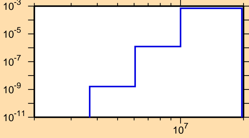
\sigma vs. E for ^{80}\text{As}(n,\alpha)
