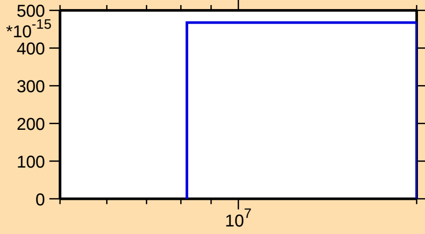
\sigma vs. E for ^{80}\text{As}(n,2n\alpha)
