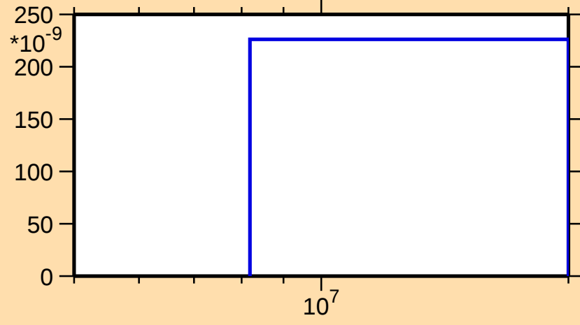
\sigma vs. E for ^{80}\text{As}(n,\text{nd})
