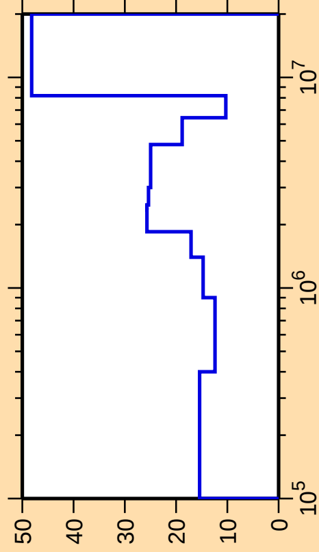
\Delta\sigma/\sigma vs. E for ^{80}\text{As}(n,\text{inel.})
