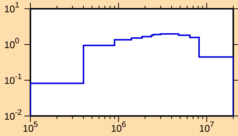
\sigma vs. E for ^{80}\text{As}(n,\text{inel.})
