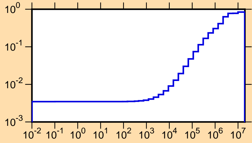
\mu vs. E for ^{201}\text{At}(\text{mt251})
