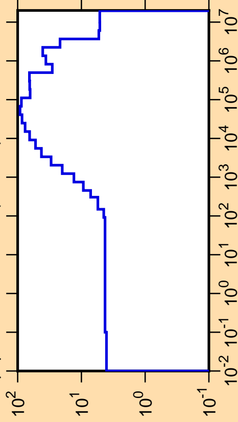
\Delta\mu/\mu vs. E for ^{201}\text{At}(\text{mt251})
