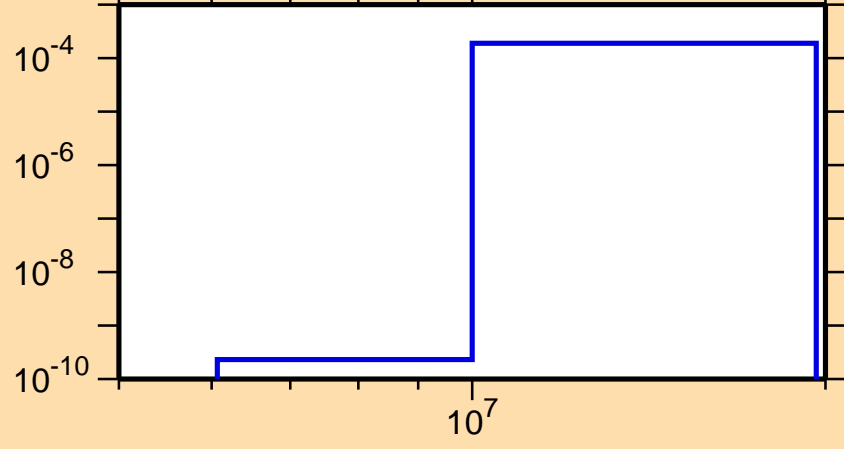
\sigma vs. E for ^{201}\text{At}(n,t)
