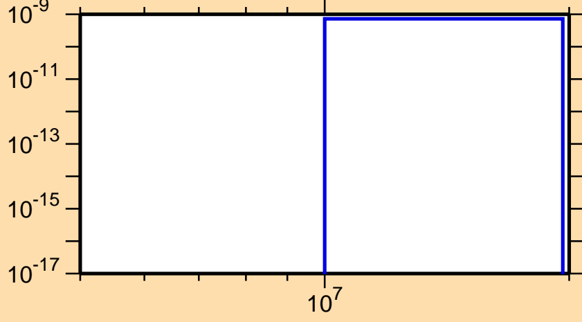
\sigma vs. E for ^{201}\text{At}(n,pd)
