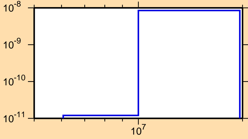
\sigma vs. E for ^{201}\text{At}(\text{mt } 45)
