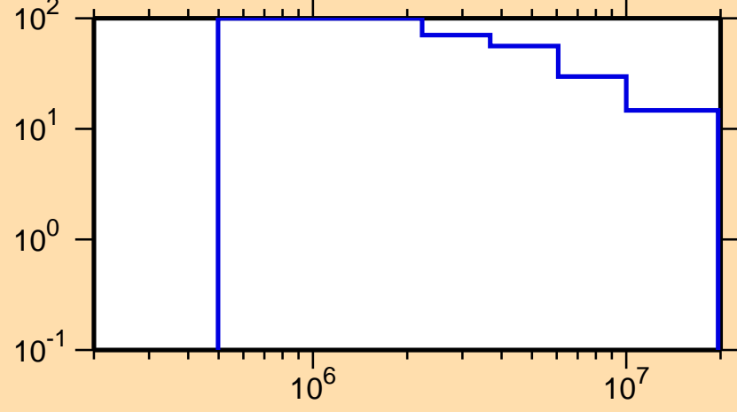
\Delta\sigma/\sigma vs. E for ^{201}\text{At}(n,\text{inel.})
