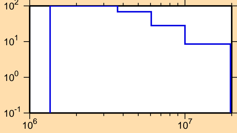
\Delta\sigma/\sigma vs. E for ^{201}\text{At}(n,n\text{cont.})
