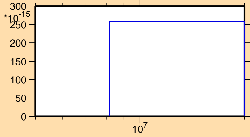
\sigma vs. E for ^{201}\text{At}(n,\text{pt})
