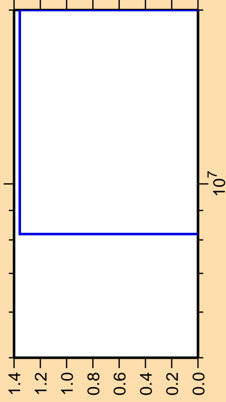
\Delta\sigma/\sigma vs. E for ^{201}\text{At}(n,\text{pt})
