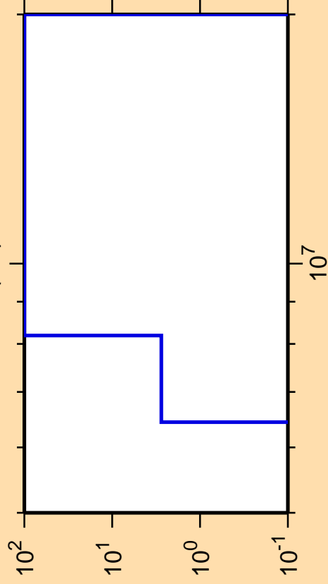
\Delta\sigma/\sigma vs. E for ^{201}\text{At}(n,t)
