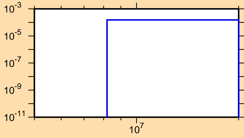
\sigma vs. E for ^{201}\text{At}(n,t)
