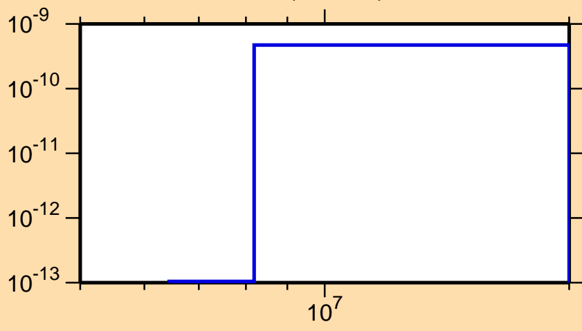
\sigma vs. E for ^{201}\text{At}(\text{mt117})
