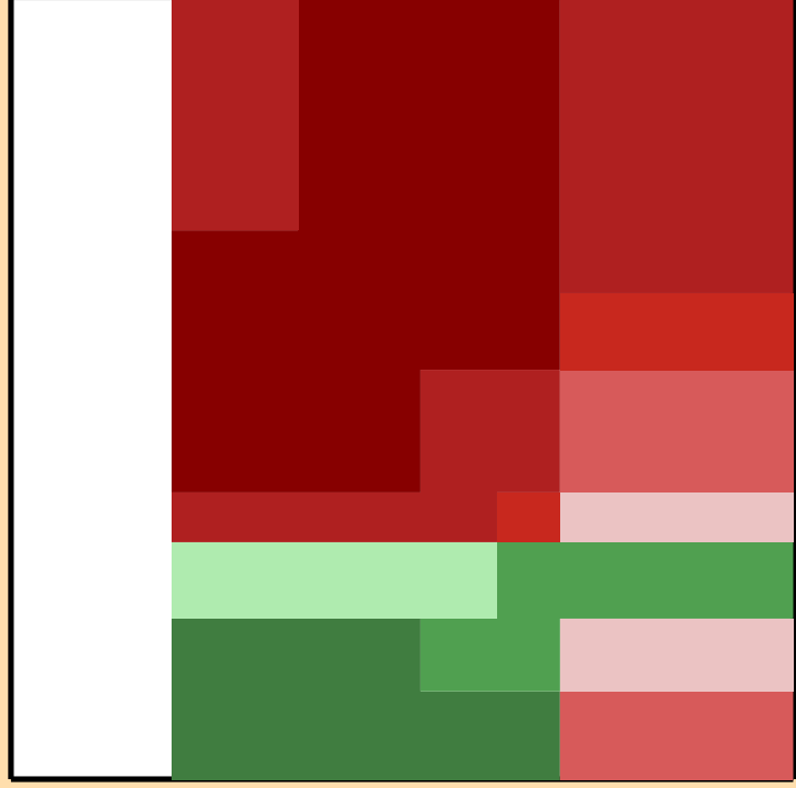
\Delta\sigma/\sigma vs. E for ^{201}\text{At}(n,n\text{cont.})
