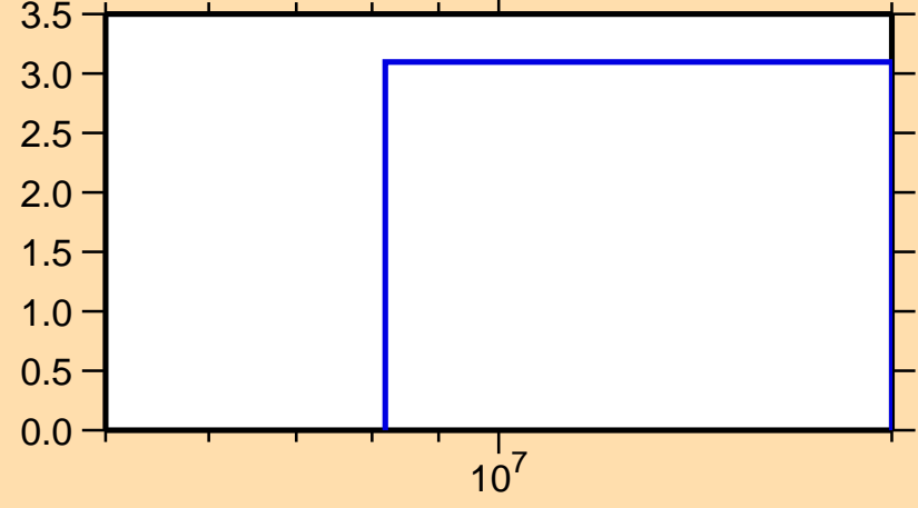
\Delta\sigma/\sigma vs. E for ^{201}\text{At}(n,\text{tot.})
