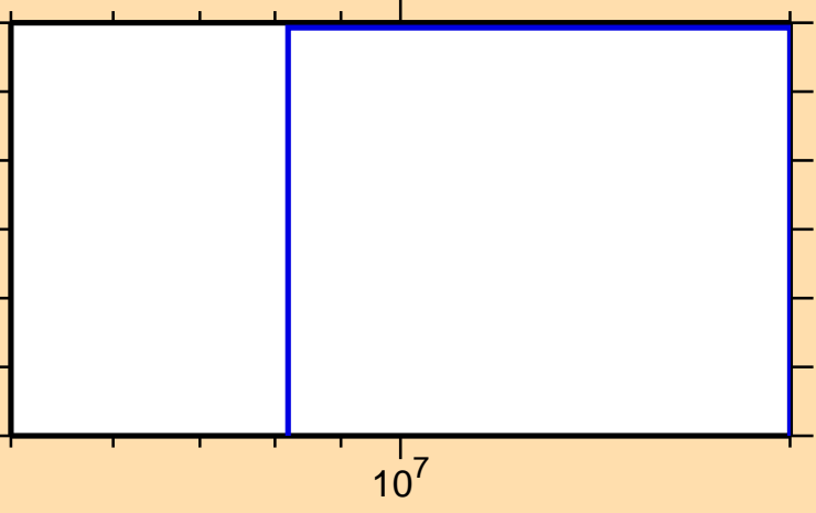
\sigma vs. E for ^{201}\text{At}(n,\text{pd})
