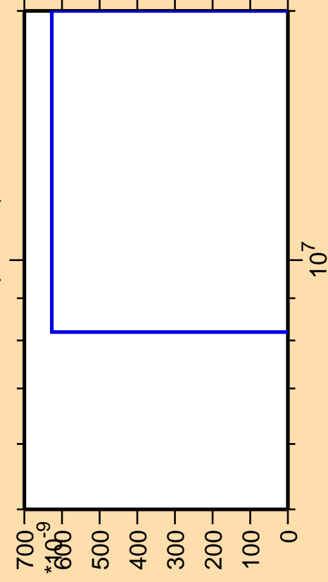
\Delta\sigma/\sigma vs. E for ^{201}\text{At}(\text{mt } 42)
