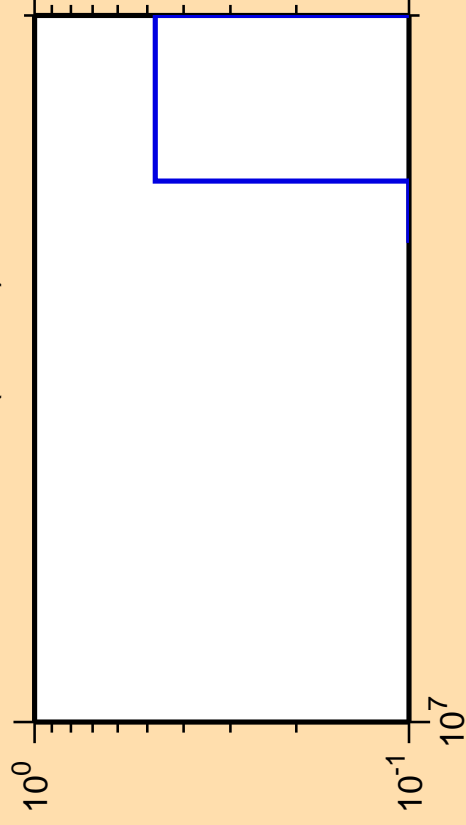
\Delta\sigma/\sigma vs. E for ^{220}\text{At} (mt 34)
