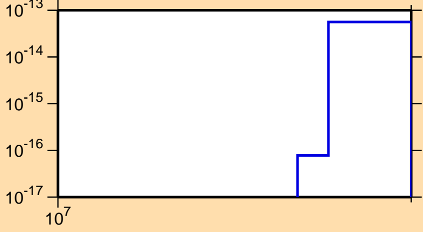
\sigma vs. E for ^{220}\text{At} (mt 34)
