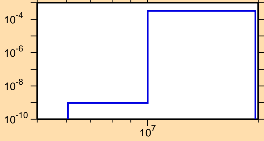
\sigma vs. E for ^{220}\text{At}(n,d)
