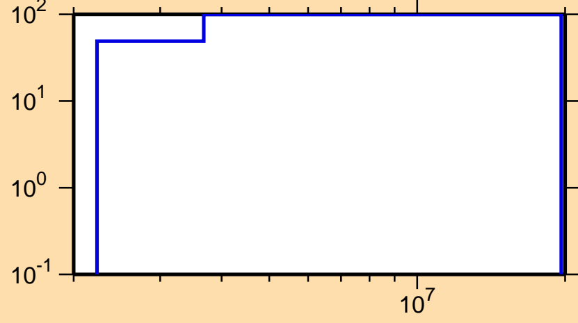
\Delta\sigma/\sigma vs. E for ^{220}\text{At}(n,ncont.)
