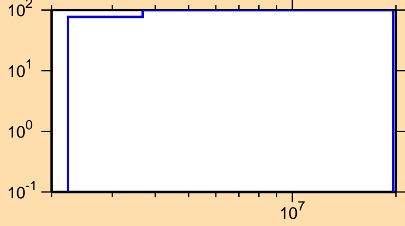
\Delta\sigma/\sigma vs. E for ^{220}\text{At}(n,p)
