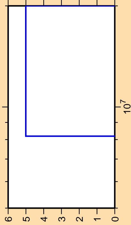
\Delta\sigma/\sigma vs. E for ^{220}\text{At}(n,p\alpha)
