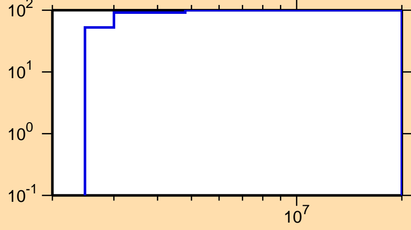
\Delta\sigma/\sigma vs. E for ^{220}\text{At}(n,\text{inel.})
