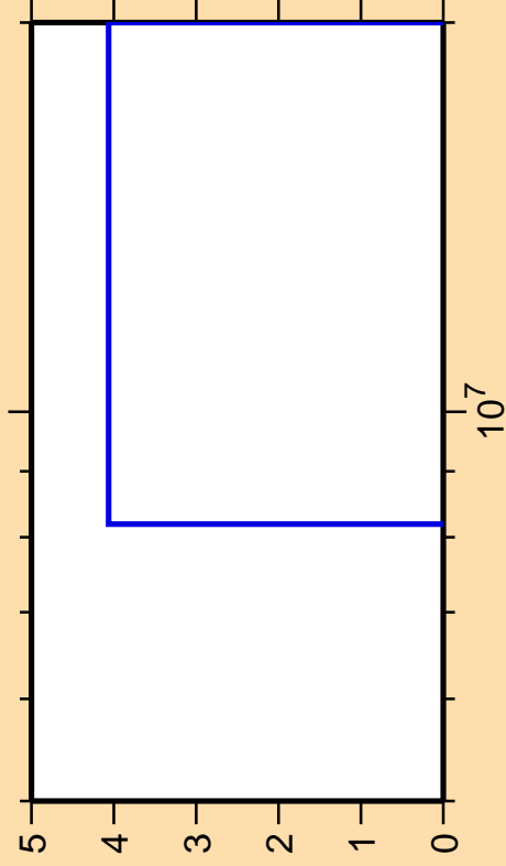
\Delta\sigma/\sigma vs. E for ^{220}\text{At}(n,\text{He}3)
