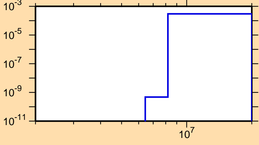
\sigma vs. E for ^{220}\text{At}(n,t)
