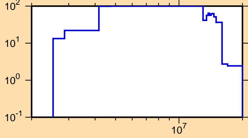
\Delta\sigma/\sigma vs. E for ^{224}\text{At}(n,ncont.)
