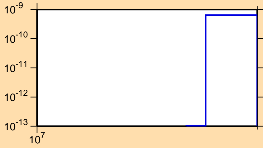
\sigma vs. E for ^{224}\text{At}(\text{mt } 11)
