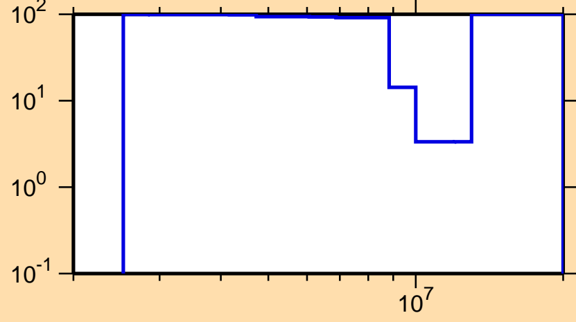
\Delta\sigma/\sigma vs. E for ^{224}\text{At}(n,\gamma)
