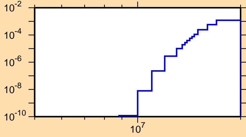
\sigma vs. E for ^{224}\text{At}(n,d)
