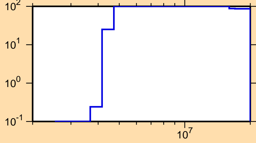
\Delta\sigma/\sigma vs. E for ^{224}\text{At}(n,p)
