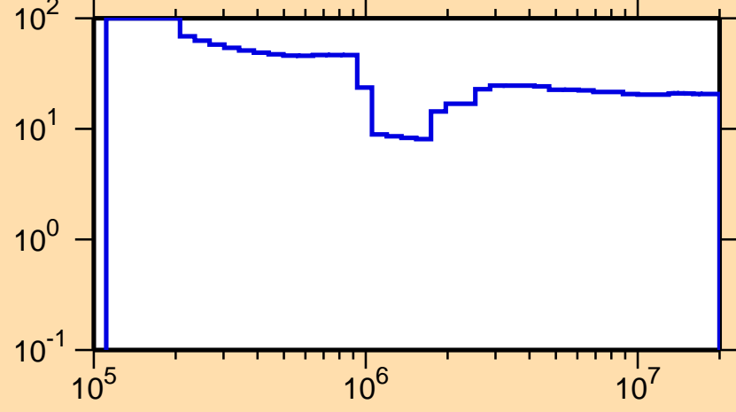
\Delta\sigma/\sigma vs. E for ^{224}\text{At}(n,\text{nonel.})
