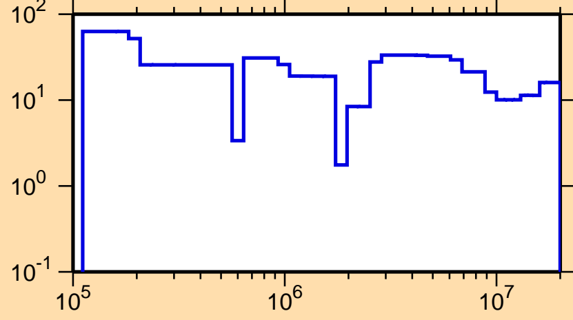
\Delta\sigma/\sigma vs. E for ^{224}\text{At}(n,\text{tot.})
