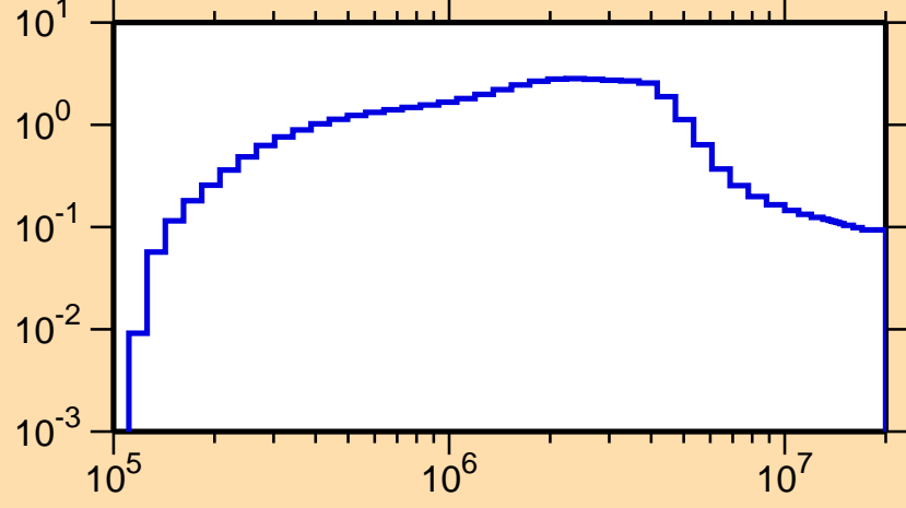
\sigma vs. E for ^{224}\text{At}(n,\text{inel.})
