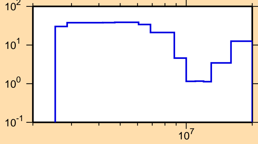
\Delta\sigma/\sigma vs. E for ^{224}\text{At}(n,el.)
