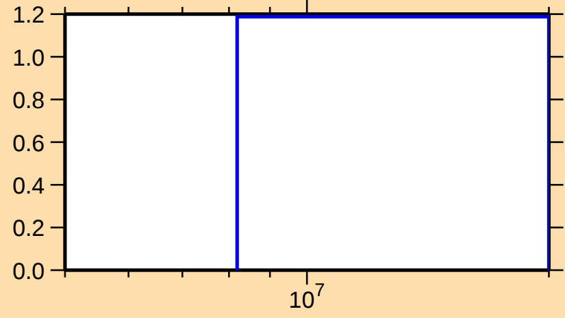
\sigma vs. E for ^{224}\text{At}(n,3n)
