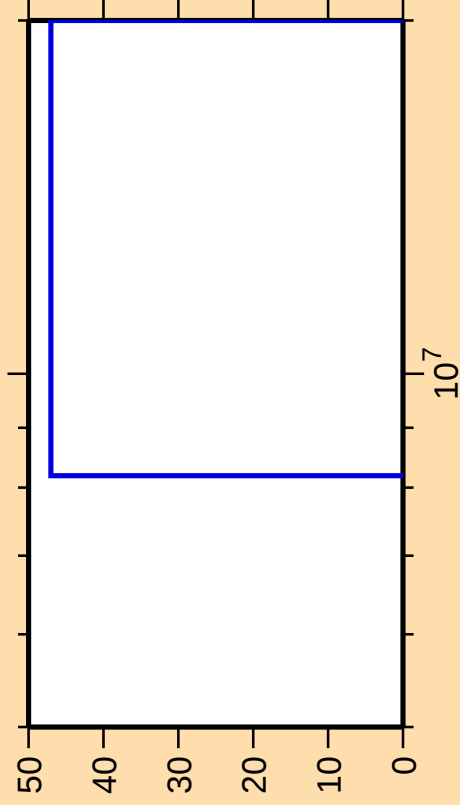
\Delta\sigma/\sigma vs. E for ^{224}\text{At}(\text{mt } 11)
