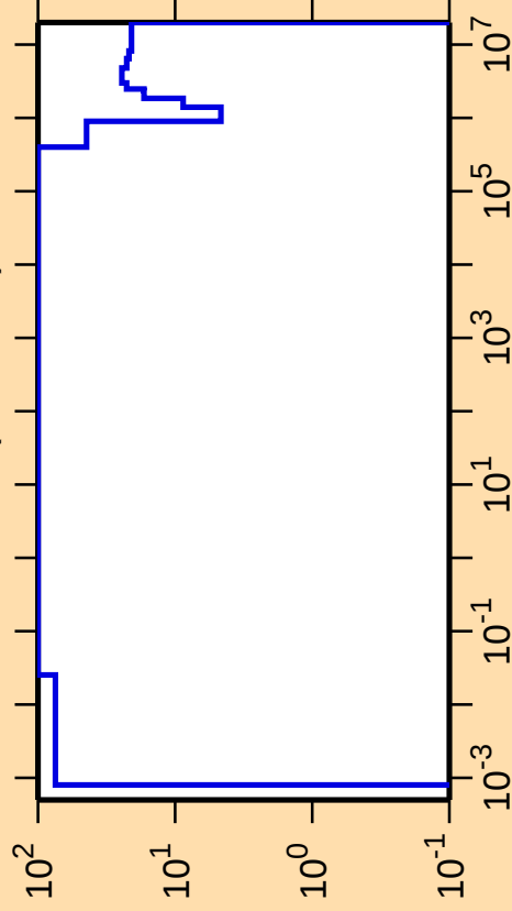
\Delta\sigma/\sigma vs. E for ^{224}\text{At}(n,\text{nonel.})
