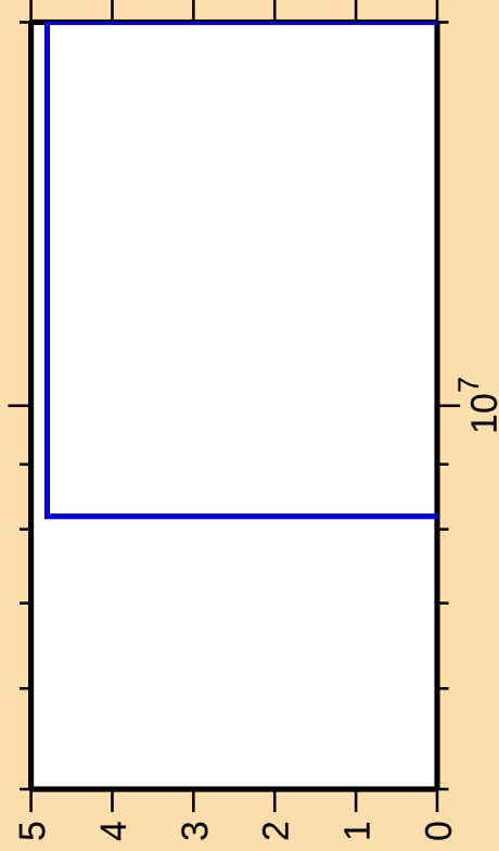
\Delta\sigma/\sigma vs. E for ^{224}\text{At}(\text{mt } 42)
