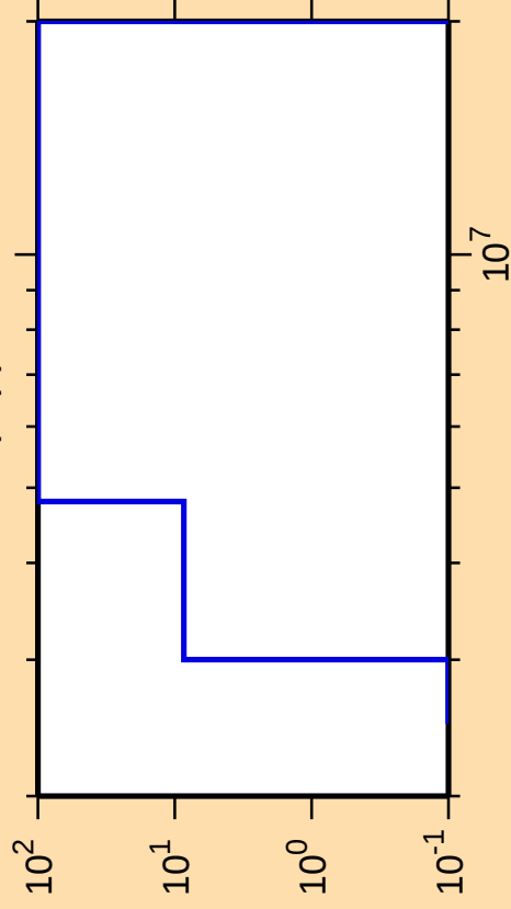
\Delta\sigma/\sigma vs. E for ^{224}\text{At}(n,p)
