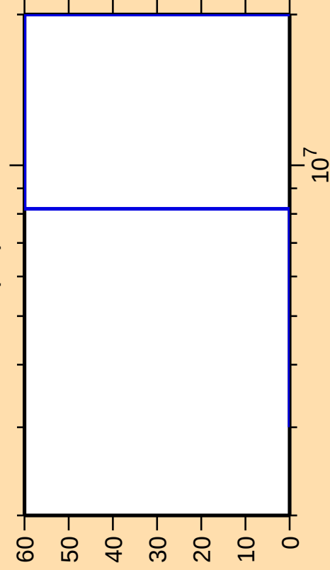
\Delta\sigma/\sigma vs. E for ^{224}\text{At}(n,f)
