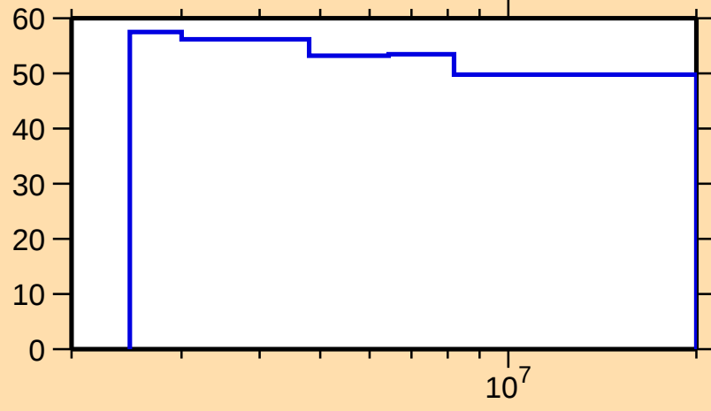
\Delta\sigma/\sigma vs. E for ^{224}\text{At}(n,n_1)
