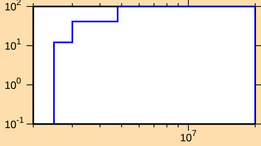
\Delta\sigma/\sigma vs. E for ^{224}\text{At}(n,n\text{cont.})
