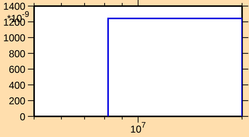
\sigma vs. E for ^{224}\text{At}(n,\text{nd})
