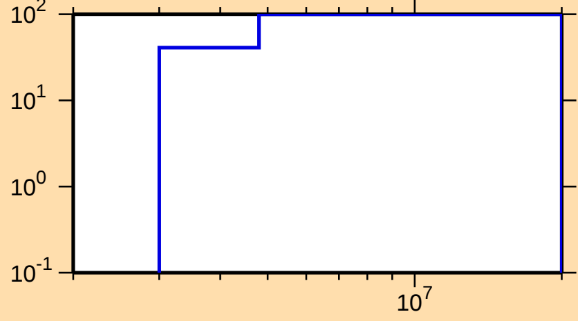
\Delta\sigma/\sigma vs. E for ^{224}\text{At}(n,\text{inel.})
