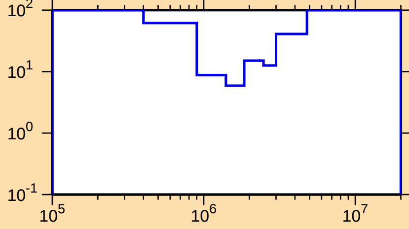
\Delta\sigma/\sigma vs. E for ^{224}\text{At}(n,\text{inel.})
