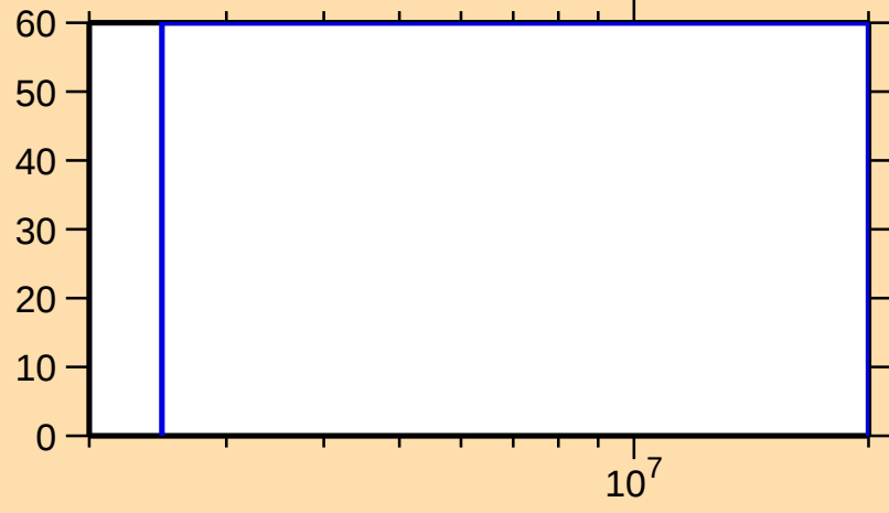
\Delta\sigma/\sigma vs. E for ^{224}\text{At}(n,\gamma)
