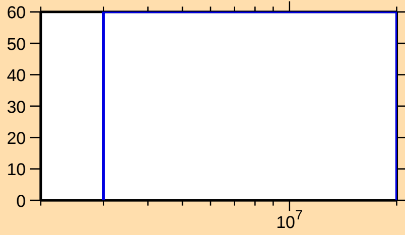
\Delta\sigma/\sigma vs. E for ^{224}\text{At}(n,2n)
