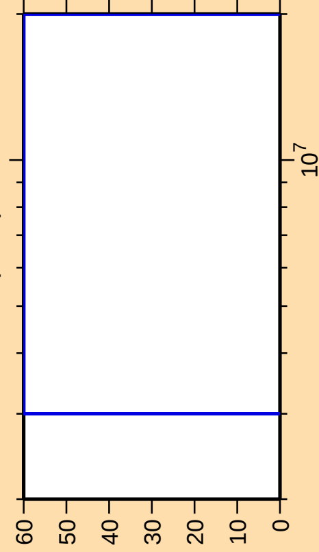
\Delta\sigma/\sigma vs. E for ^{224}\text{At}(n,2n)
