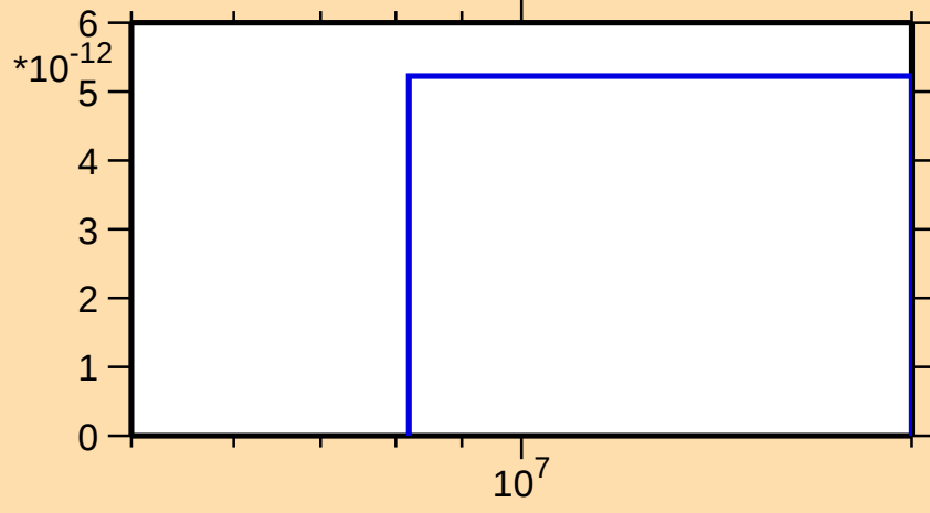
\sigma vs. E for ^{224}\text{At}(\text{mt } 11)
