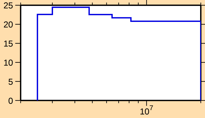
\Delta\sigma/\sigma vs. E for ^{224}\text{At}(n,\text{nonel.})
