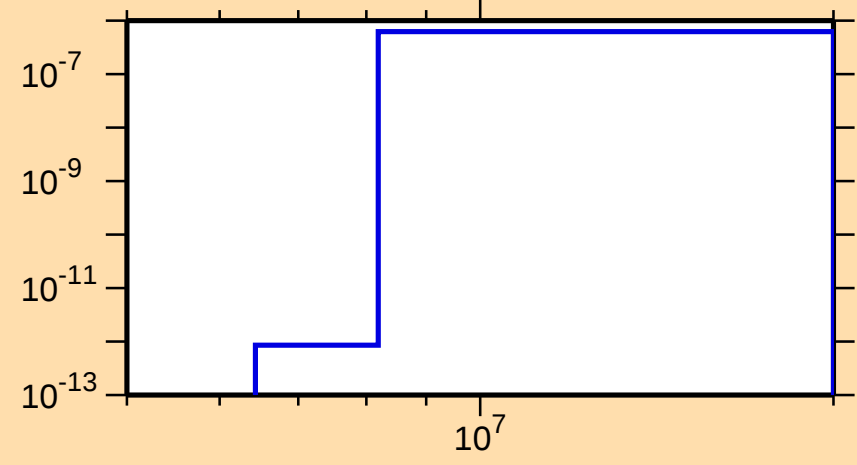
\sigma vs. E for ^{224}\text{At}(n,2n\alpha)
