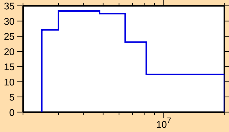
\Delta\sigma/\sigma vs. E for ^{224}\text{At}(n,\text{tot.})
