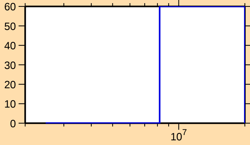
\Delta\sigma/\sigma vs. E for ^{224}\text{At}(n,f)
