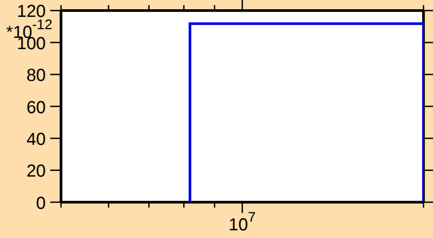
\sigma vs. E for ^{224}\text{At}(n,3n\alpha)
