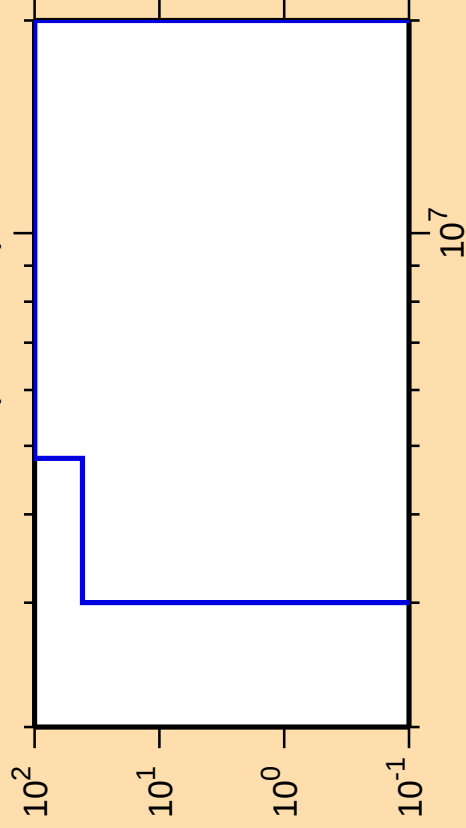
\Delta\sigma/\sigma vs. E for ^{224}\text{At}(n,n\text{cont.})
