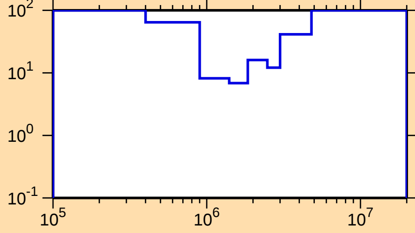
\Delta\sigma/\sigma vs. E for ^{224}\text{At}(n,\text{ncont.})
