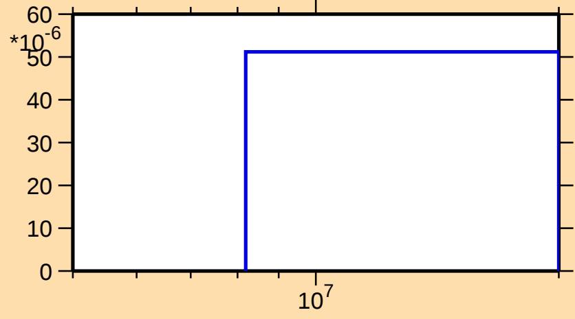
\sigma vs. E for ^{224}\text{At}(n,np)
