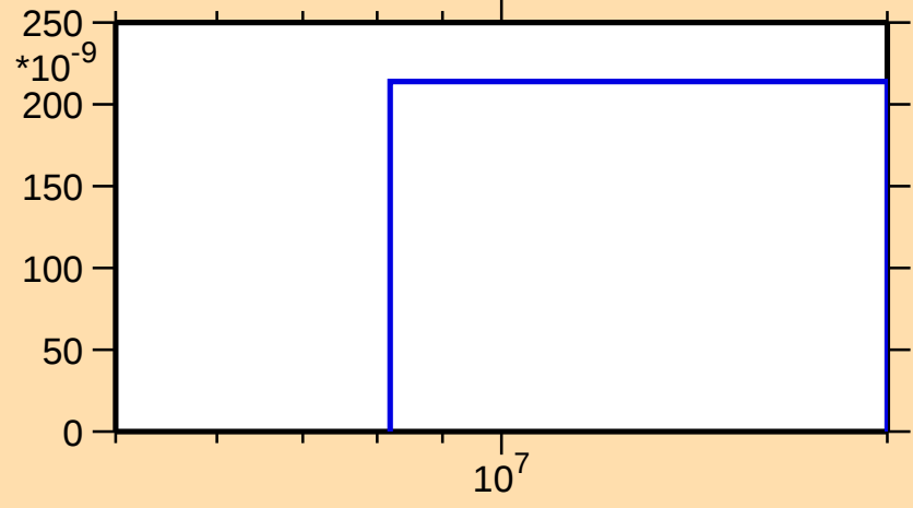
\sigma vs. E for ^{224}\text{At}(n,2np)
