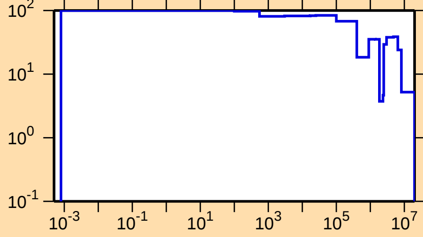
\Delta\sigma/\sigma vs. E for ^{224}\text{At}(n,\text{el.})
