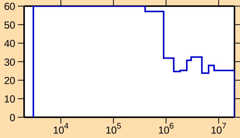
\Delta\sigma/\sigma vs. E for ^{176}\text{Au}(n,n\text{nonel.})
