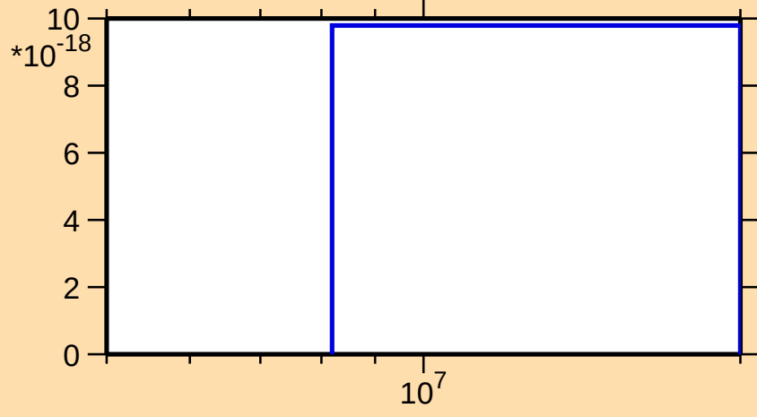
\sigma vs. E for ^{176}\text{Au}(\text{mt } 42)
