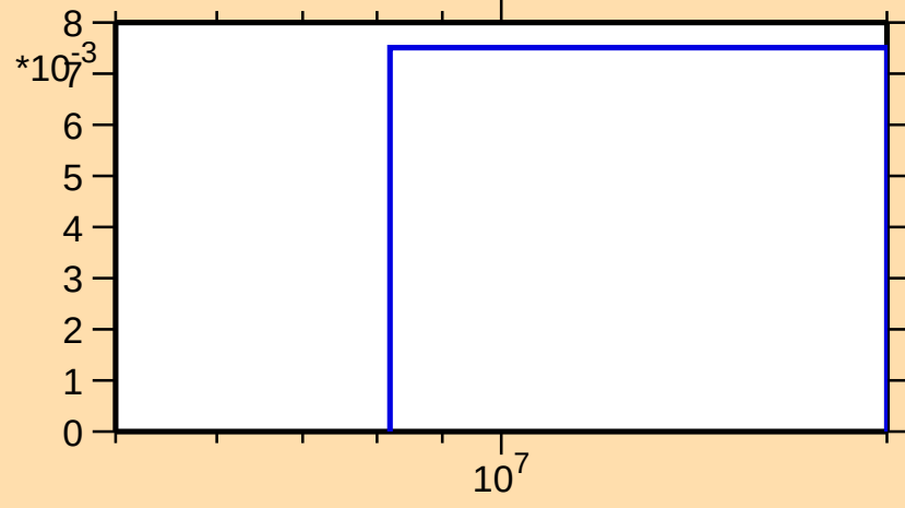
\sigma vs. E for ^{176}\text{Au}(n,2n\alpha)
