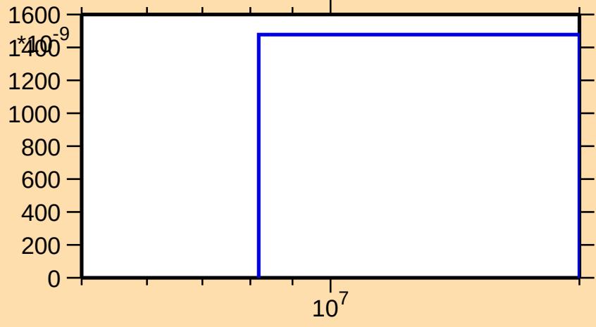
\sigma vs. E for ^{176}\text{Au}(n,\text{pt})
