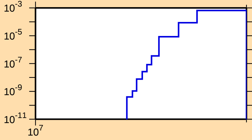
\sigma vs. E for ^{185}\text{Au}(n,2np)
