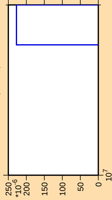
\Delta\sigma/\sigma vs. E for ^{185}\text{Au}(\text{mt } 42)
