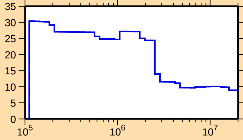
\Delta\sigma/\sigma vs. E for ^{185}\text{Au}(n,n\text{nonel.})
