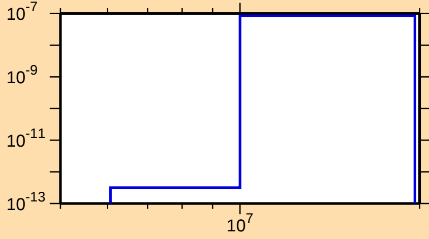
\sigma vs. E for ^{185}\text{Au}(\text{mt } 45)
