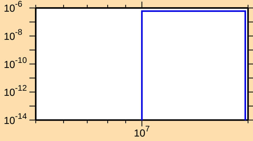
\sigma vs. E for ^{185}\text{Au}(n,2n\alpha)
