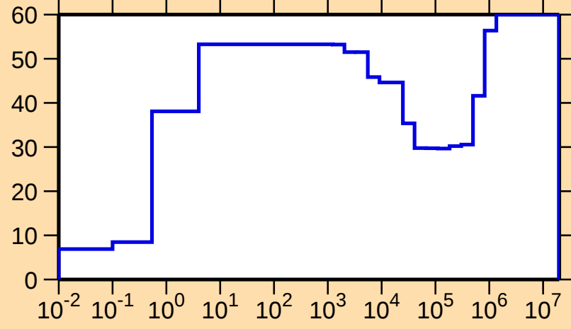
\Delta\sigma/\sigma vs. E for ^{185}\text{Au}(n,\gamma)
