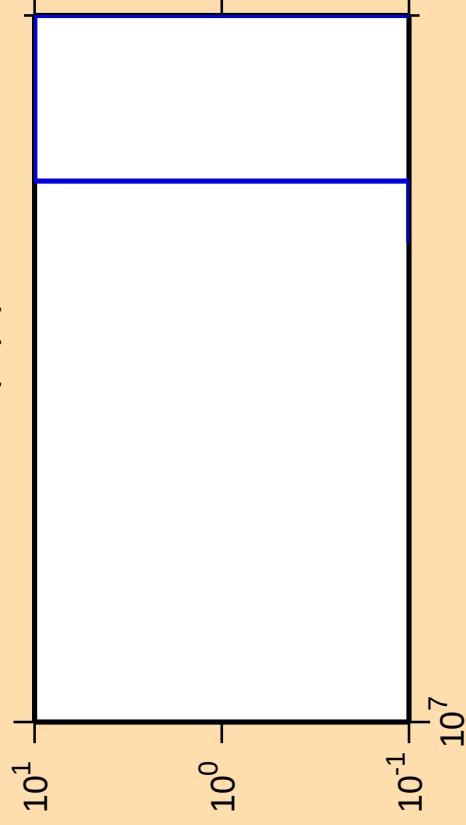
\Delta\sigma/\sigma vs. E for ^{190}\text{Au}(n,\text{pt})
