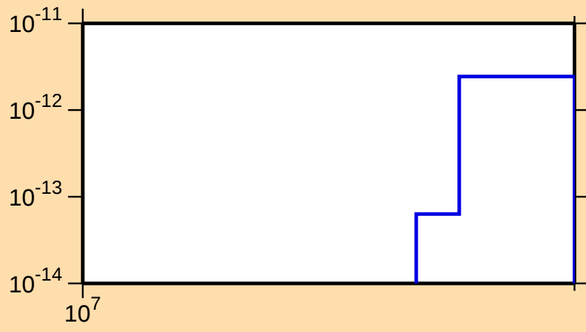
\sigma vs. E for ^{190}\text{Au}(n,\text{pd})
