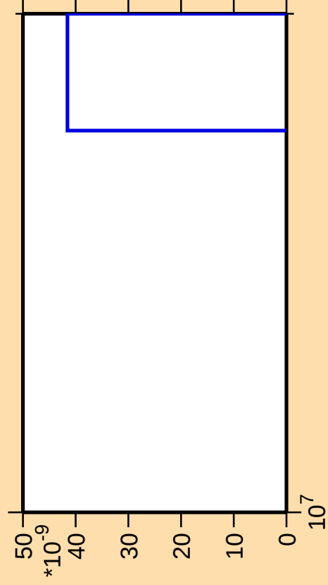
\Delta\sigma/\sigma vs. E for ^{190}\text{Au}(\text{mt } 42)
