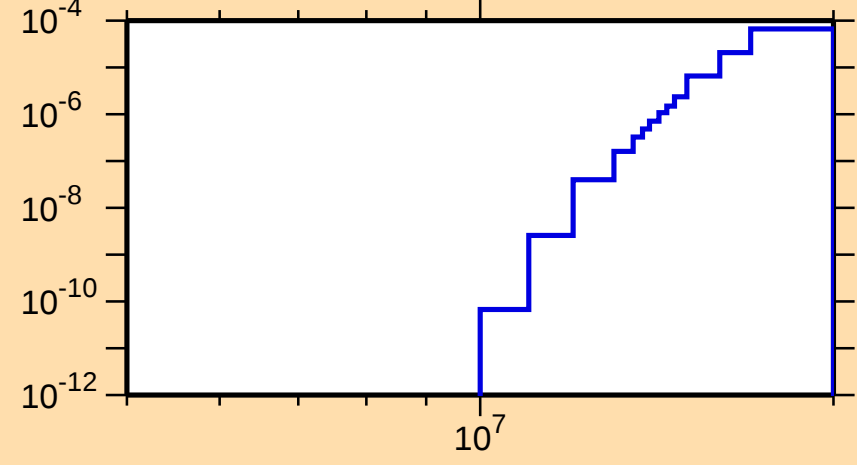
\sigma vs. E for ^{190}\text{Au}(n,2n\alpha)
