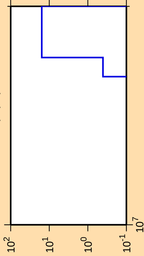
\Delta\sigma/\sigma vs. E for ^{190}\text{Au}(n,\text{pd})
