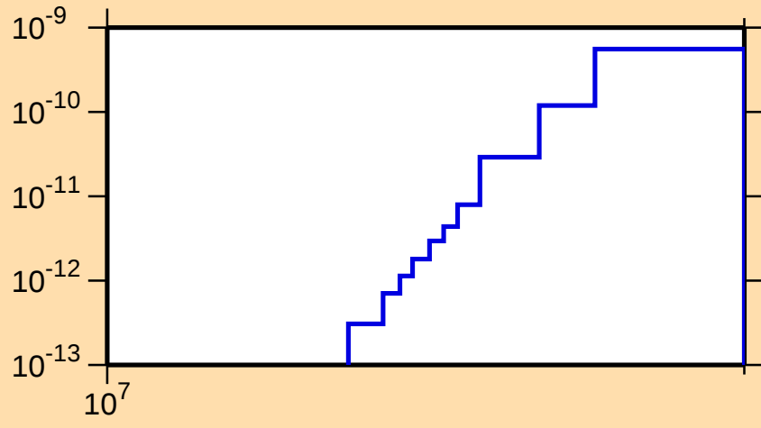
\sigma vs. E for ^{190}\text{Au}(\text{mt117})
