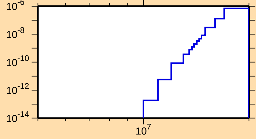
\sigma vs. E for ^{190}\text{Au}(n,\text{He3})
