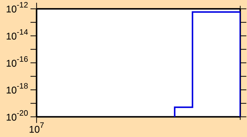
\sigma vs. E for ^{190}\text{Au}(n,3n\alpha)
