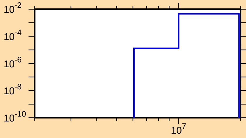
\sigma vs. E for ^{190}\text{Au}(n,np)
