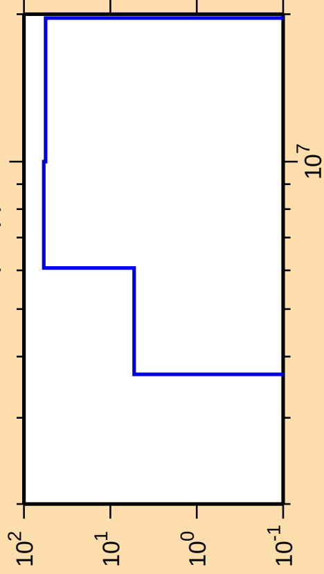
\Delta\sigma/\sigma vs. E for ^{190}\text{Au}(n,np)
