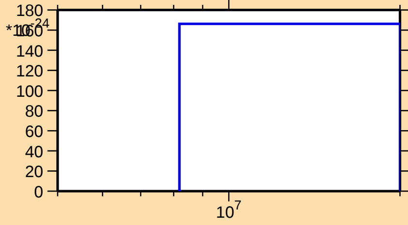
\sigma vs. E for ^{190}\text{Au}(\text{mt } 42)
