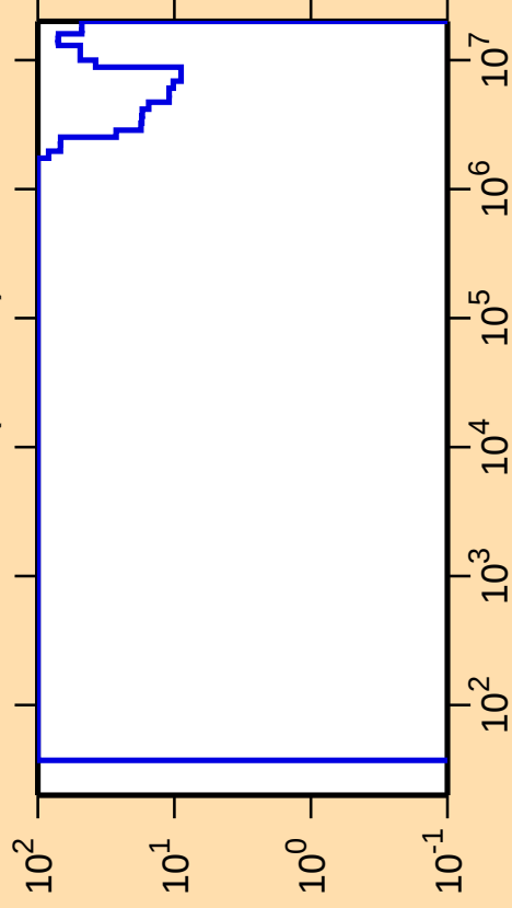
\Delta\sigma/\sigma vs. E for ^{193}\text{Au}(n,\text{inel.})
