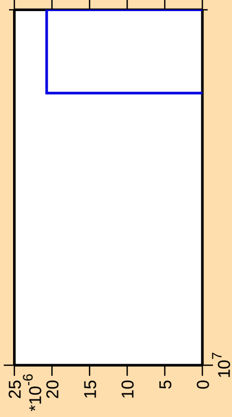
\Delta\sigma/\sigma vs. E for ^{193}\text{Au}(\text{mt } 42)
