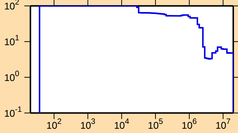
\Delta\sigma/\sigma vs. E for ^{193}\text{Au}(n,\text{nonel.})
