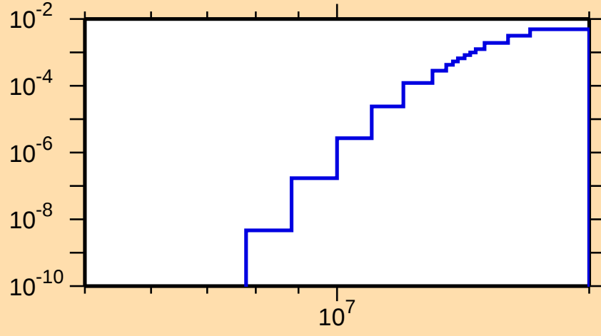
\sigma vs. E for ^{193}\text{Au}(n,d)
