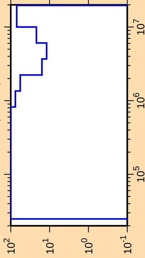
\Delta\sigma/\sigma vs. E for ^{194}\text{Au}(n,\text{inel.})
