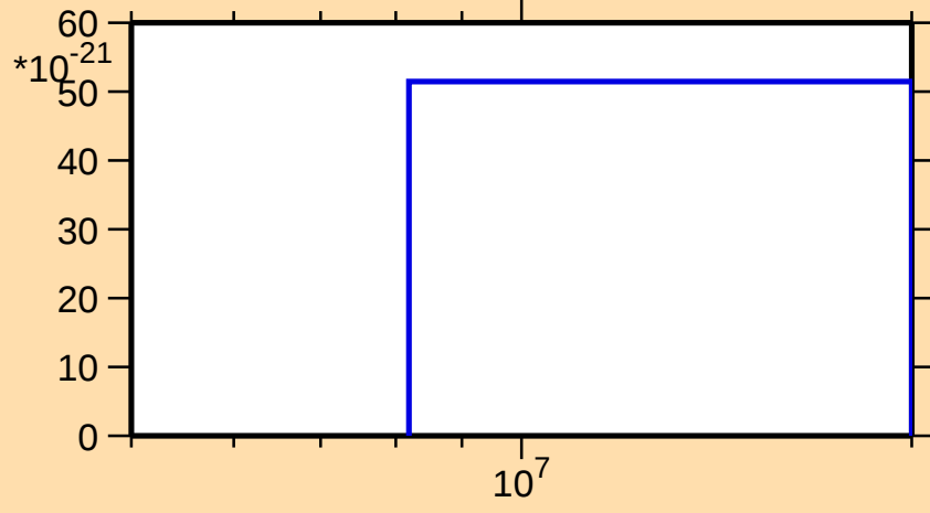
\sigma vs. E for ^{195}\text{Au}(\text{mt } 42)
