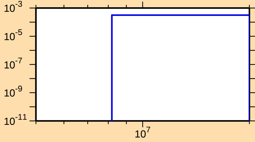
\sigma vs. E for ^{195}\text{Au}(n,d)
