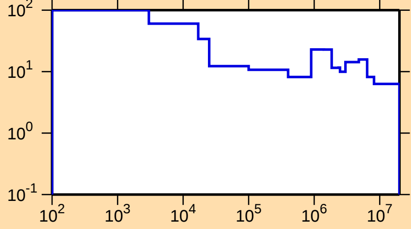
\Delta\sigma/\sigma vs. E for ^{195}\text{Au}(n,\text{el.})
