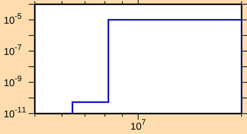
\sigma vs. E for ^{195}\text{Au}(n,n\alpha)
