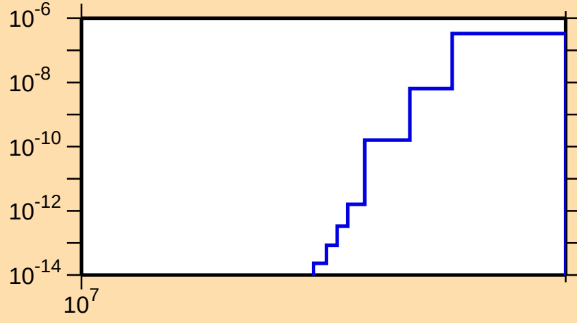
\sigma vs. E for ^{198}\text{Au}(n,2np)
