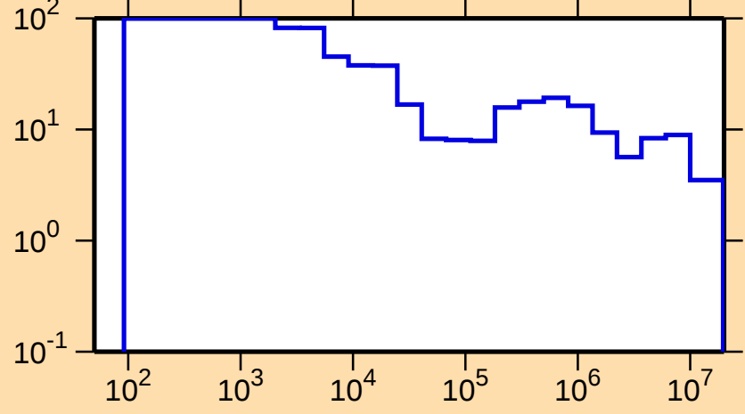
\Delta\sigma/\sigma vs. E for ^{198}\text{Au}(n,\text{tot.})
