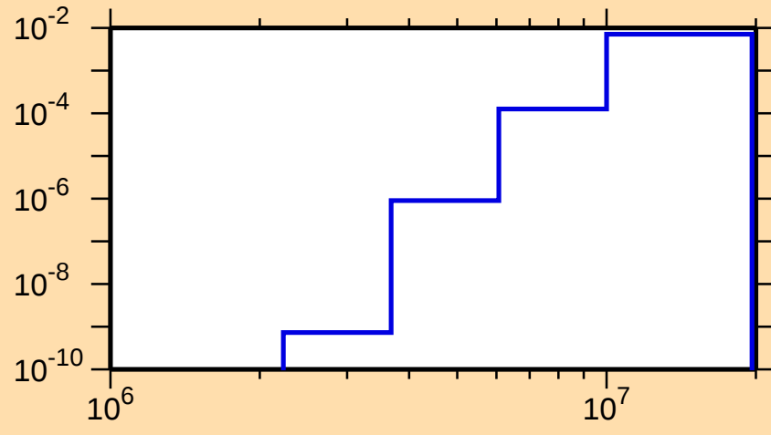
\sigma vs. E for ^{198}\text{Au}(n,p)
