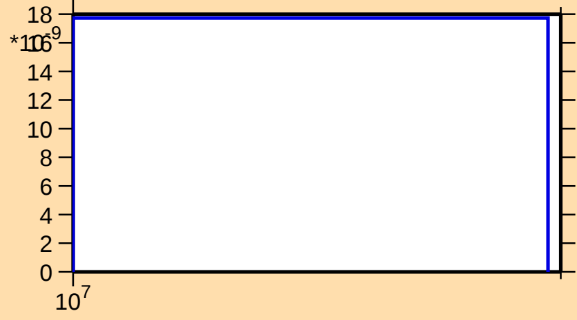
\sigma vs. E for ^{198}\text{Au}(n,\text{nd})
