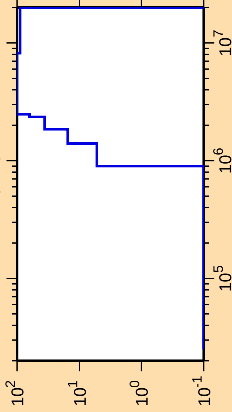
\Delta\sigma/\sigma vs. E for ^{198}\text{Au}(n,\alpha)
