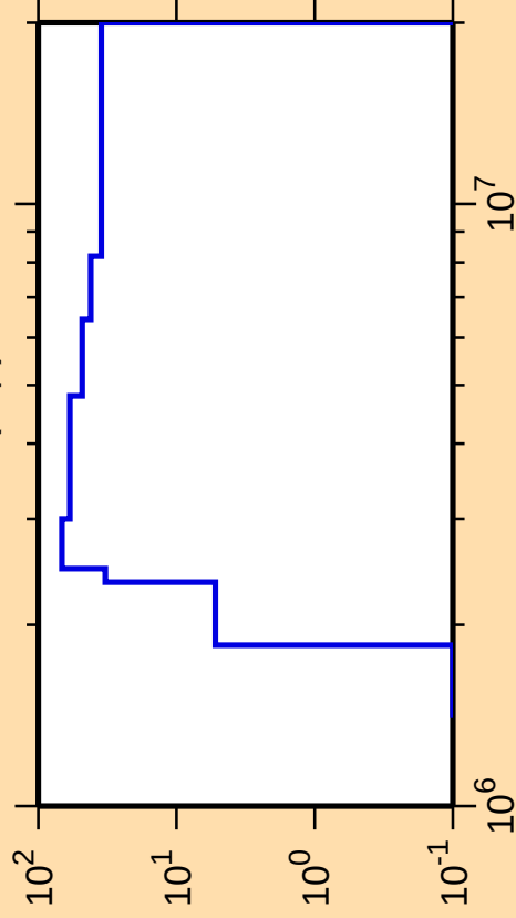
\Delta\sigma/\sigma vs. E for ^{198}\text{Au}(n,p)
