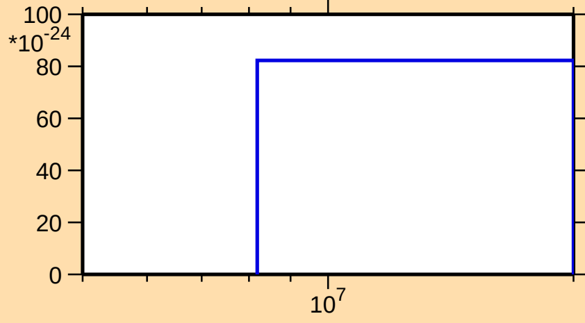
\sigma vs. E for ^{198}\text{Au}(\text{mt } 42)
