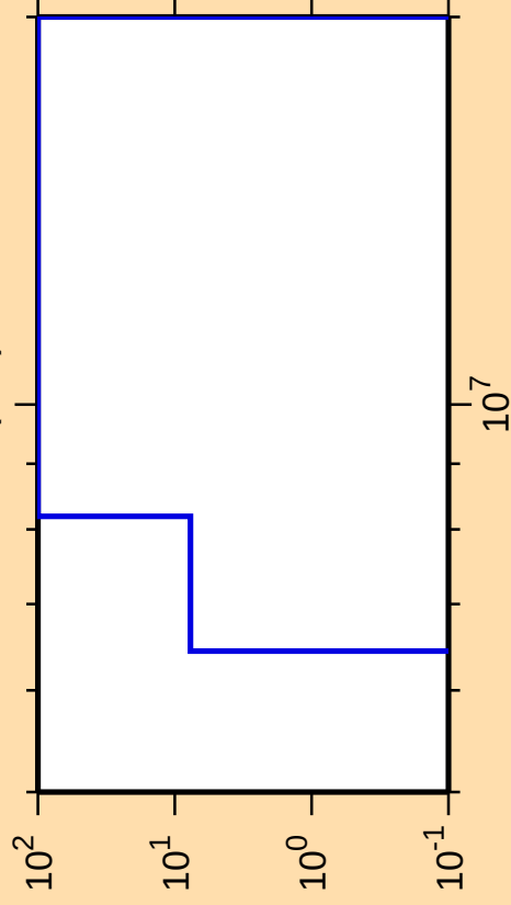
\Delta\sigma/\sigma vs. E for ^{198}\text{Au}(n,d)
