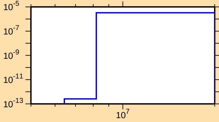
\sigma vs. E for ^{198}\text{Au}(n,n\alpha)
