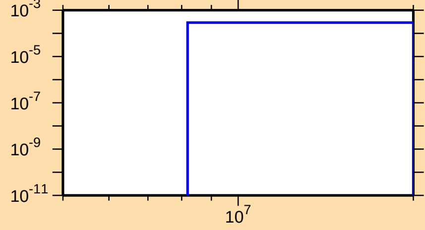
\sigma vs. E for ^{198}\text{Au}(n,d)
