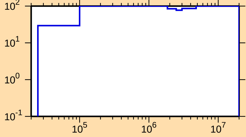
\Delta\sigma/\sigma vs. E for ^{198}\text{Au}(n,n_1)
