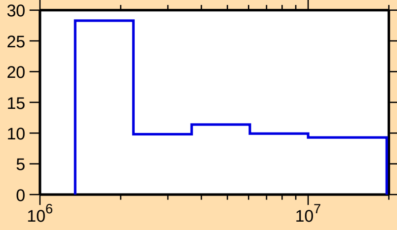
\Delta\sigma/\sigma vs. E for ^{201}\text{Au}(n,n\text{nonel.})
