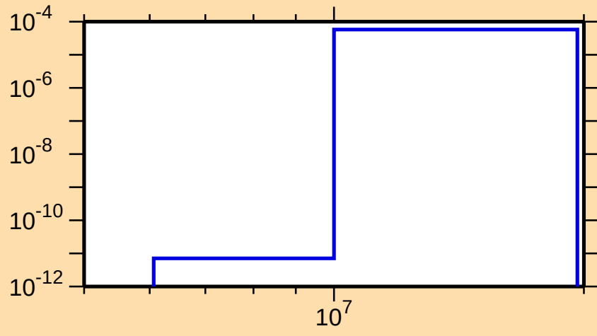
\sigma vs. E for ^{201}\text{Au}(n,d)
