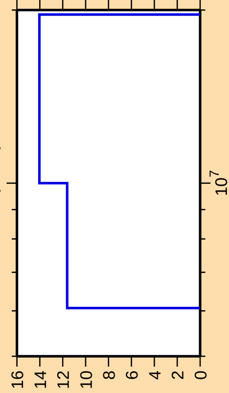
\Delta\sigma/\sigma vs. E for ^{201}\text{Au}(n,2n)
