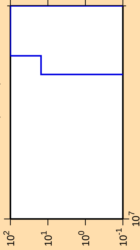
\Delta\sigma/\sigma vs. E for ^{127}\text{Ba}(\text{mt } 45)
