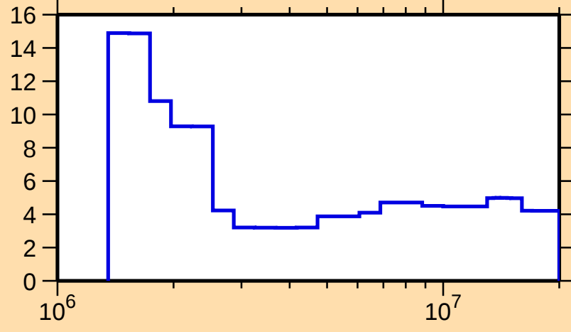
\Delta\sigma/\sigma vs. E for ^{127}\text{Ba}(n,n\text{onel.})
