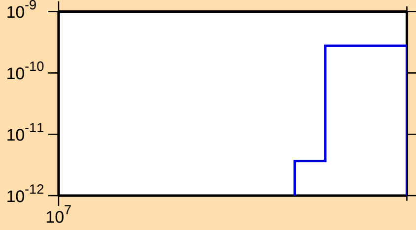
\sigma vs. E for ^{127}\text{Ba}(\text{mt } 45)
