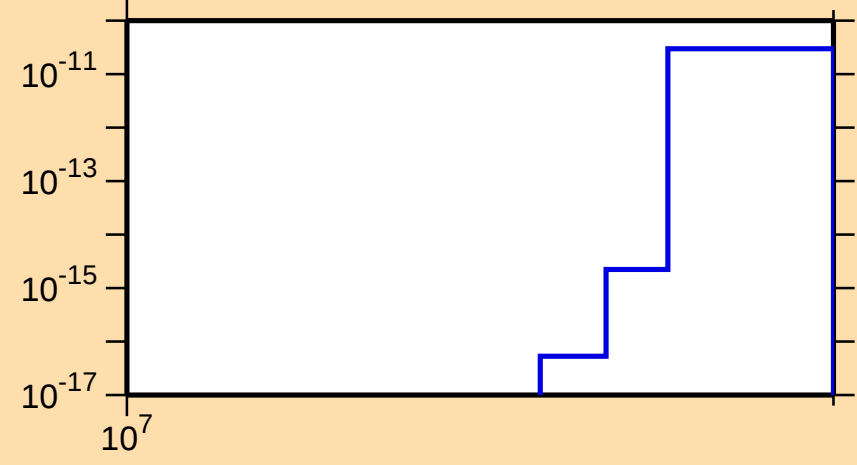
\sigma vs. E for ^{129}\text{Ba}(n,\text{nt})
