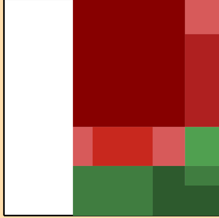
\Delta\sigma/\sigma vs. E for ^{129}\text{Ba}(n,2n)
