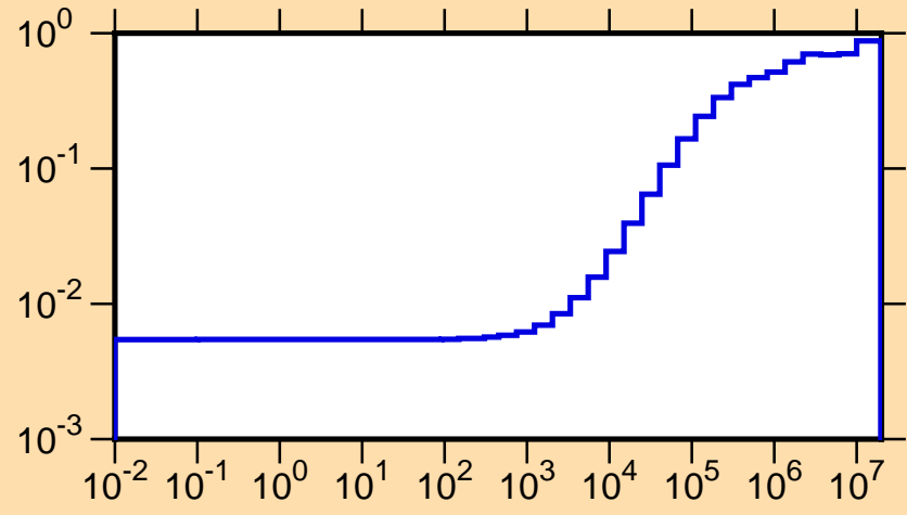
\mu vs. E for ^{129}\text{Ba}(\text{mt251})
