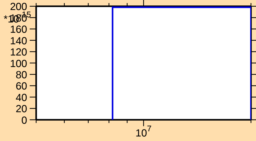
\sigma vs. E for ^{129}\text{Ba}(\text{mt } 34)
