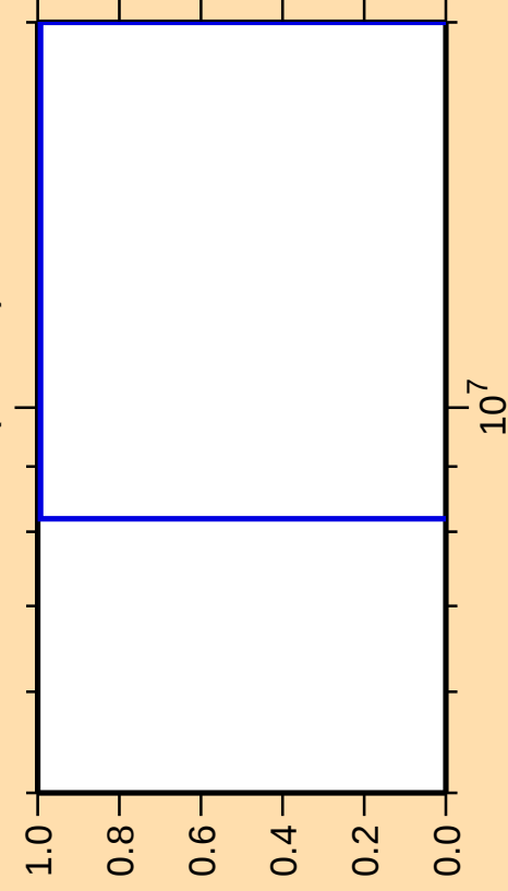
\Delta\sigma/\sigma vs. E for ^{129}\text{Ba}(\text{mt } 34)
