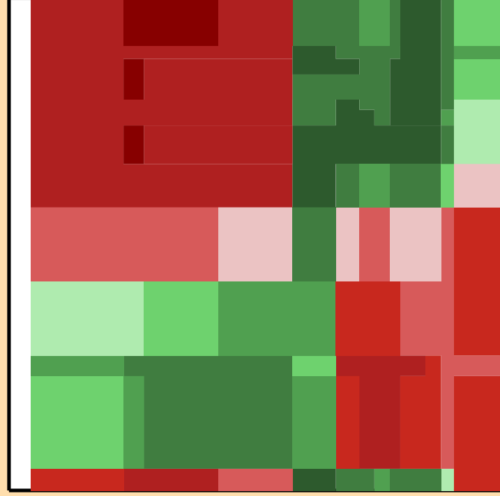
\Delta\sigma/\sigma vs. E for ^{129}\text{Ba}(n,n_1)
