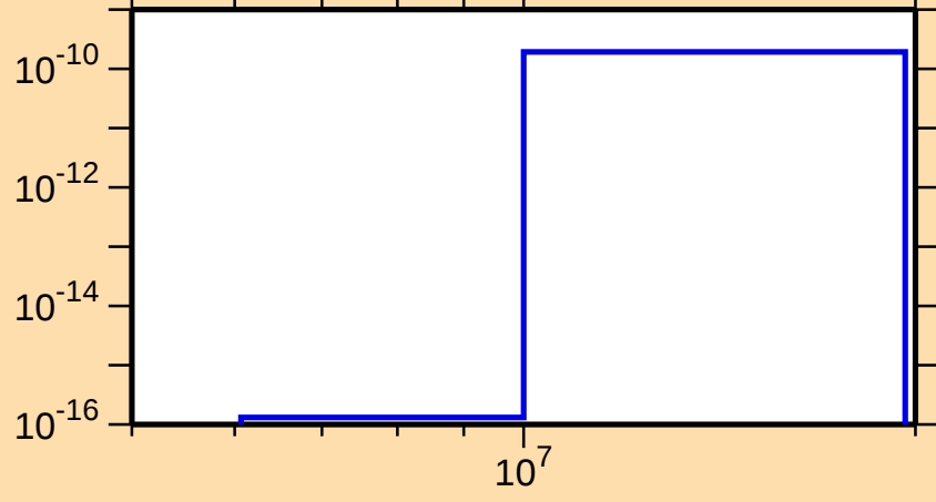
\sigma vs. E for ^{133}\text{Ba}(n,p\alpha)
