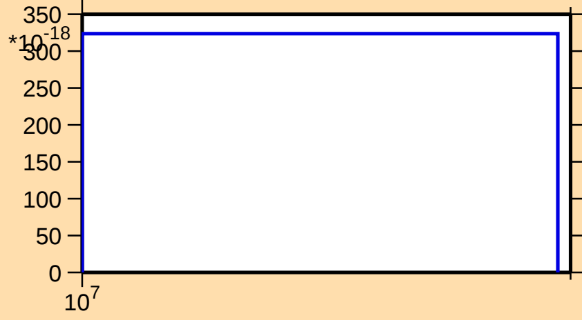
\sigma vs. E for ^{133}\text{Ba}(\text{mt } 34)
