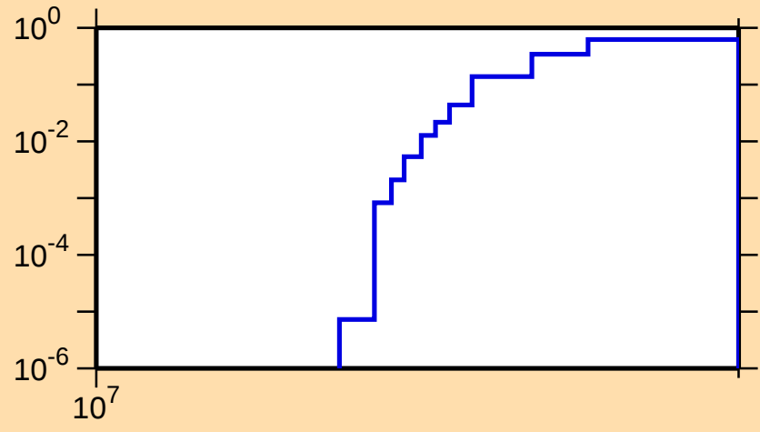
\sigma vs. E for ^{139}\text{Ba}(n,3n)
