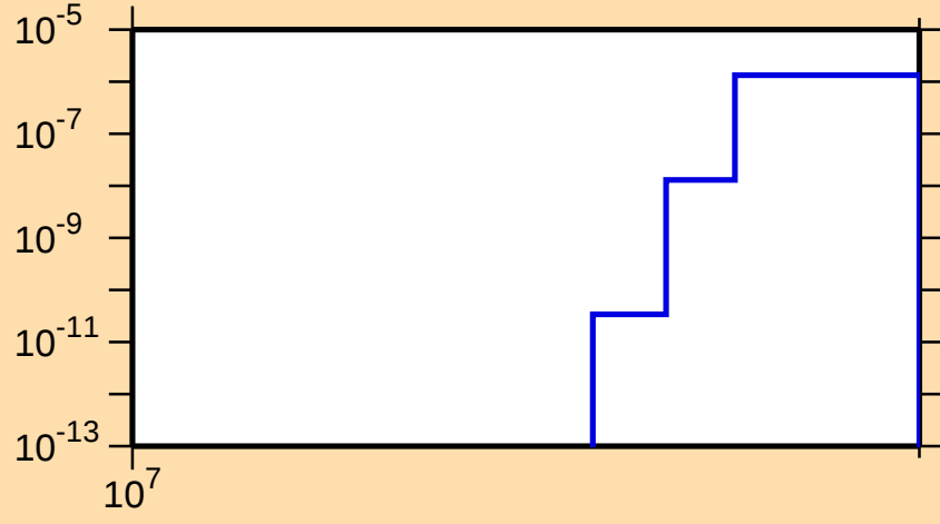
\sigma vs. E for ^{139}\text{Ba}(n,2np)
