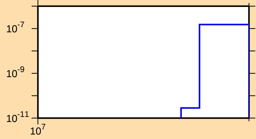
\sigma vs. E for ^{139}\text{Ba}(n,\text{nt})
