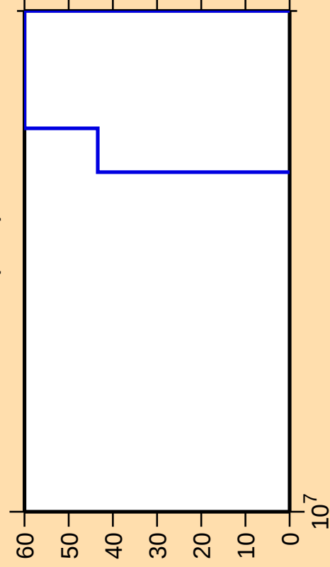
\Delta\sigma/\sigma vs. E for ^{139}\text{Ba}(n,\text{nt})
