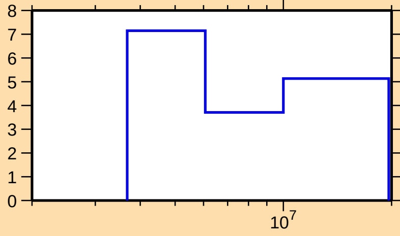
\Delta\sigma/\sigma vs. E for ^{139}\text{Ba}(n,\text{tot.})
