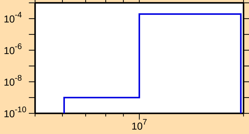
\sigma vs. E for ^{139}\text{Ba}(n,n\alpha)
