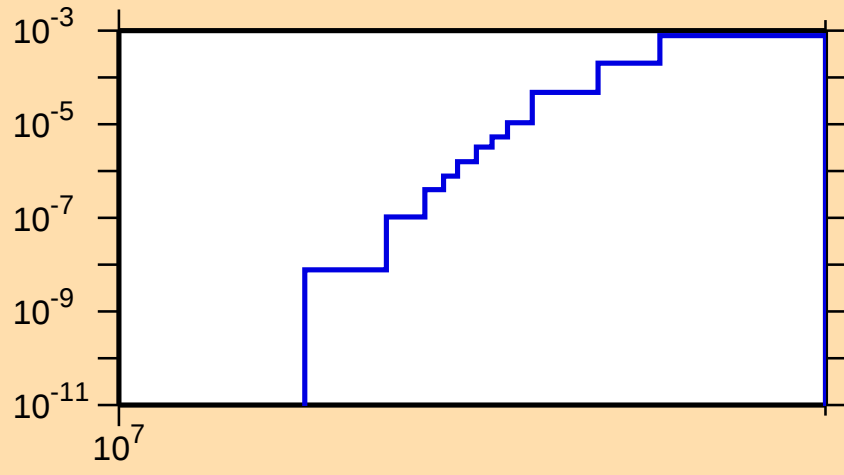
\sigma vs. E for ^{141}\text{Ba}(n,np)
