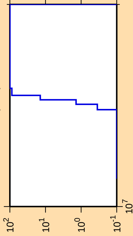
\Delta\sigma/\sigma vs. E for ^{141}\text{Ba}(n,\text{nt})
