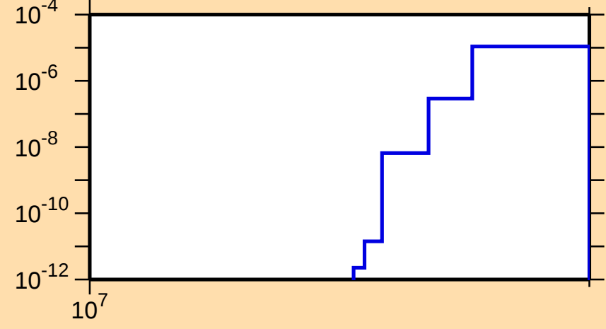
\sigma vs. E for ^{141}\text{Ba}(n,\text{nt})
