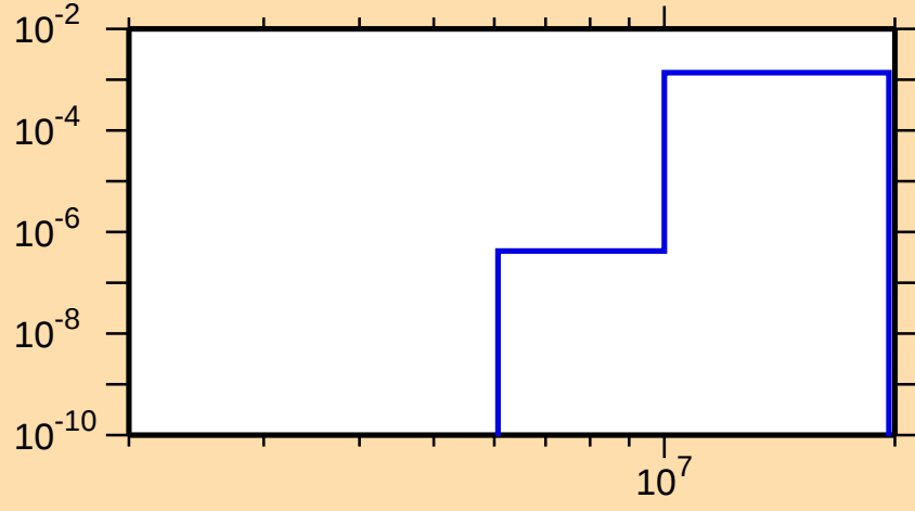
\sigma vs. E for ^{141}\text{Ba}(n,p)
