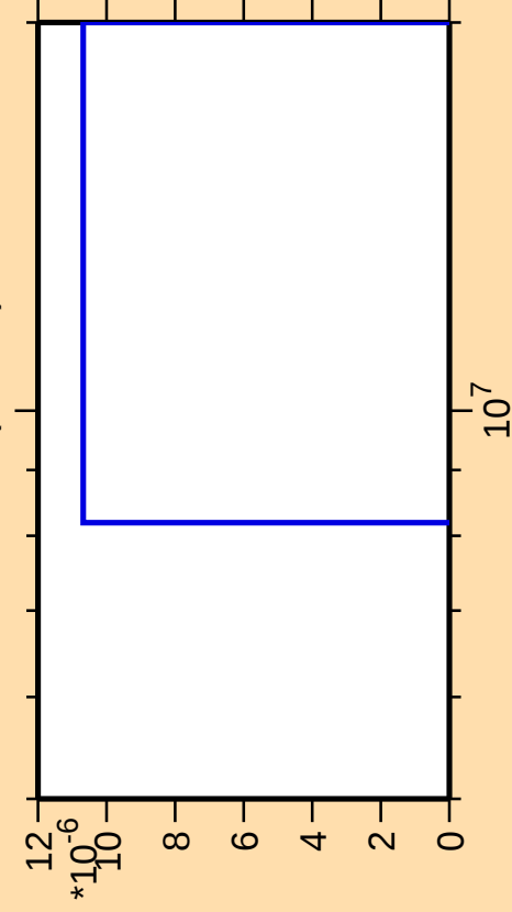
\Delta\sigma/\sigma vs. E for ^{141}\text{Ba}(\text{mt } 11)
