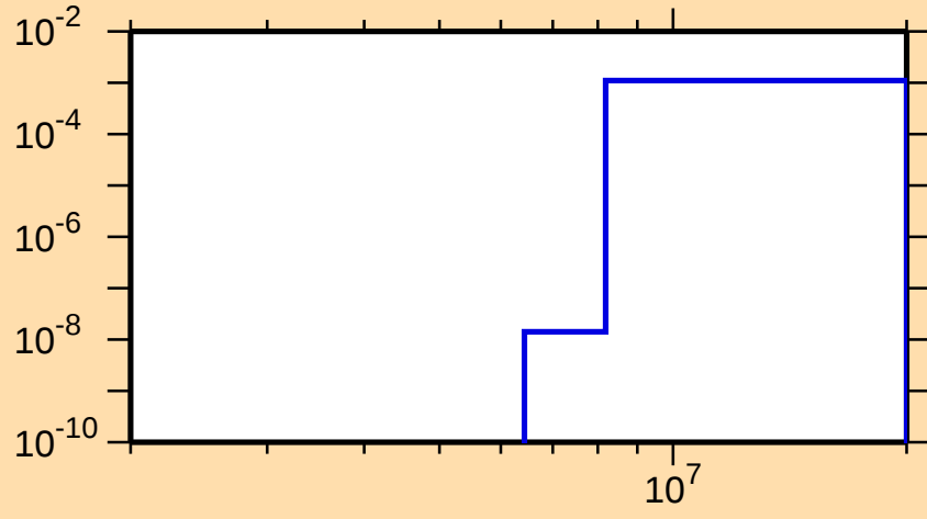
\sigma vs. E for ^{141}\text{Ba}(n,p)
