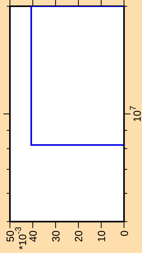
\Delta\sigma/\sigma vs. E for ^{141}\text{Ba}(n,3n\alpha)
