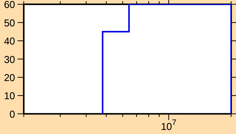
\Delta\sigma/\sigma vs. E for ^{141}\text{Ba}(n,n\text{cont.})
