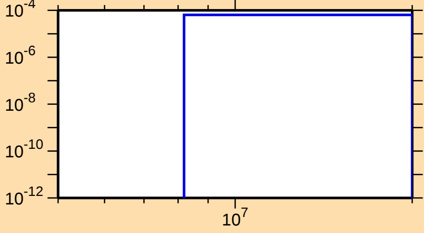
\sigma vs. E for ^{141}\text{Ba}(n,d)
