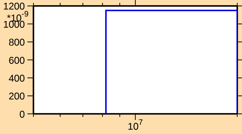
\sigma vs. E for ^{141}\text{Ba}(n,2n\alpha)
