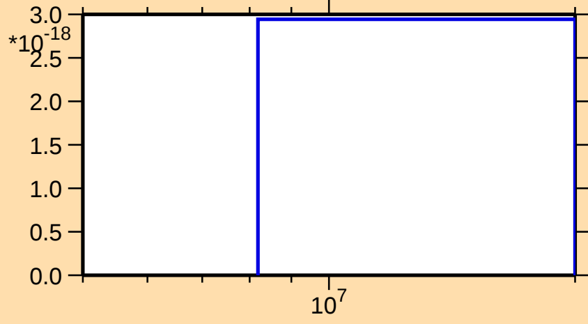
\sigma vs. E for ^{141}\text{Ba}(\text{mt } 11)
