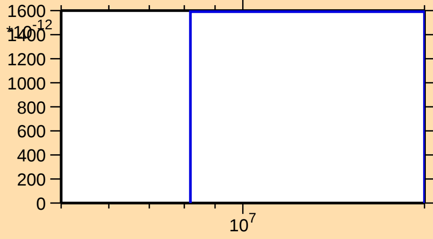
\sigma vs. E for ^{141}\text{Ba}(n,2np)
