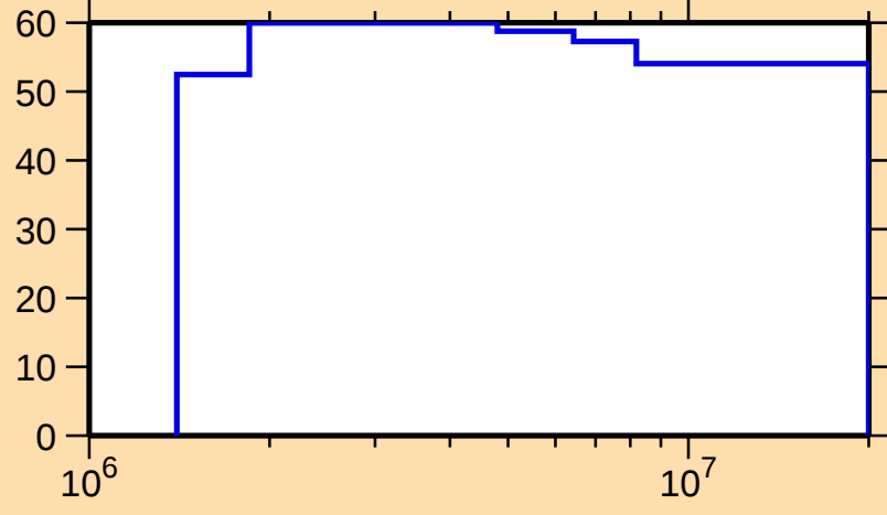
\Delta\sigma/\sigma vs. E for ^{141}\text{Ba}(n,n_1)
