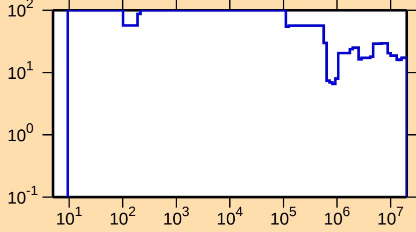
\Delta\sigma/\sigma vs. E for ^{144}\text{Ba}(n,\text{tot.})
