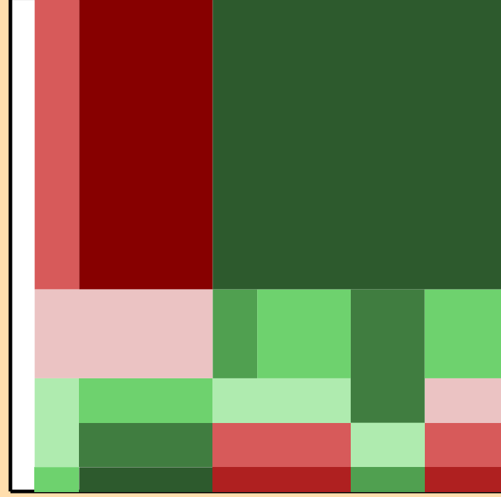
\Delta\sigma/\sigma vs. E for ^{144}\text{Ba}(n,2n)
