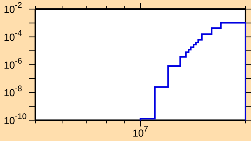
\sigma vs. E for ^{144}\text{Ba}(n,p)
