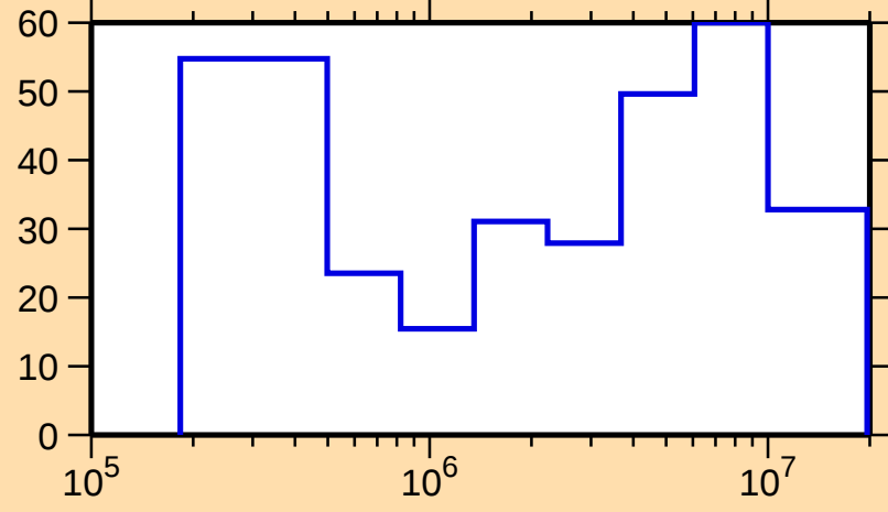
\Delta\sigma/\sigma vs. E for ^{144}\text{Ba}(\text{n,el.})
