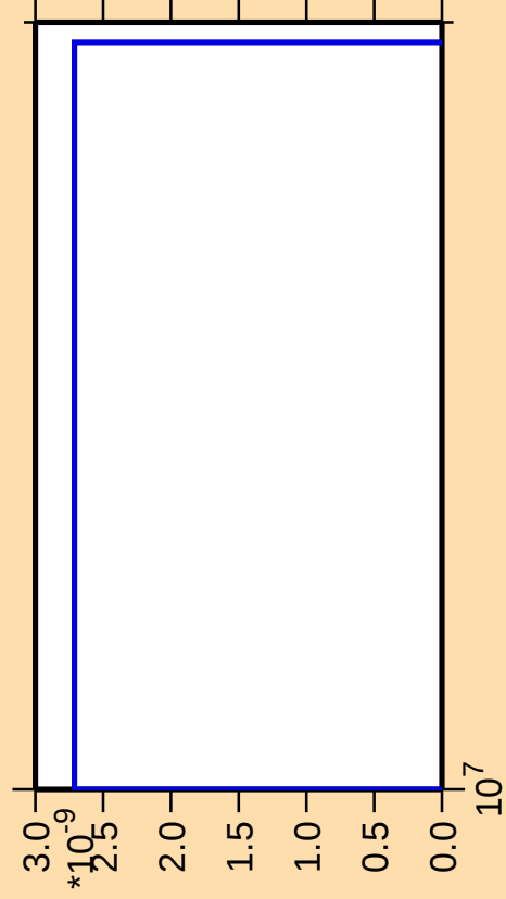
\Delta\sigma/\sigma vs. E for ^{144}\text{Ba}(\text{mt } 11)
