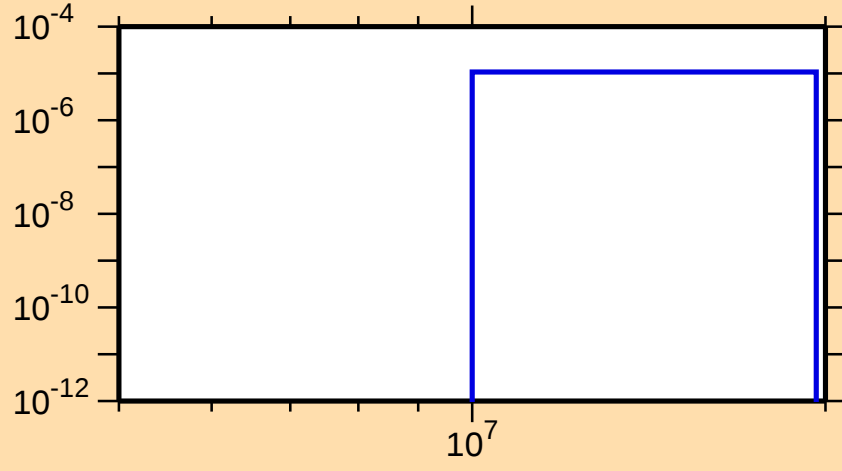
\sigma vs. E for ^{144}\text{Ba}(n,t)
