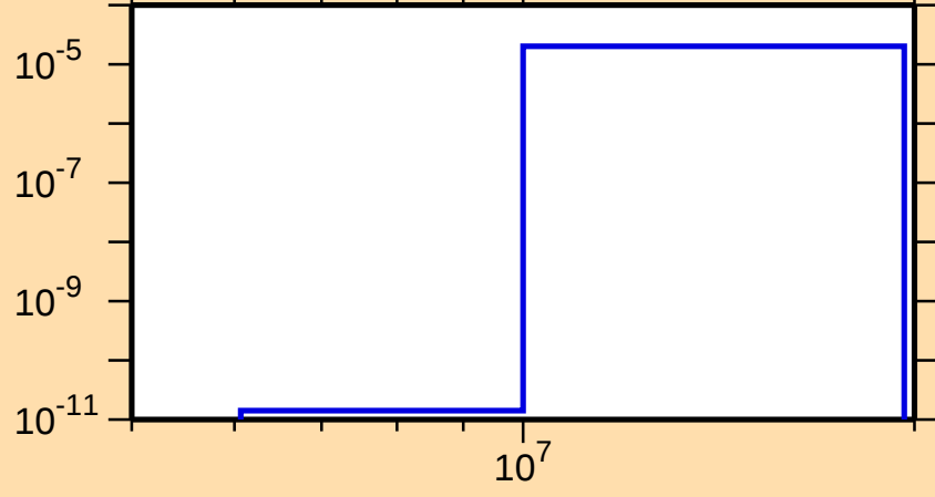
\sigma vs. E for ^{144}\text{Ba}(n,n\alpha)
