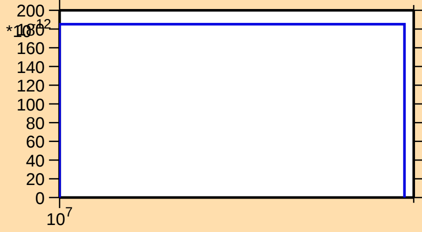
\sigma vs. E for ^{144}\text{Ba}(n,\text{nd})
