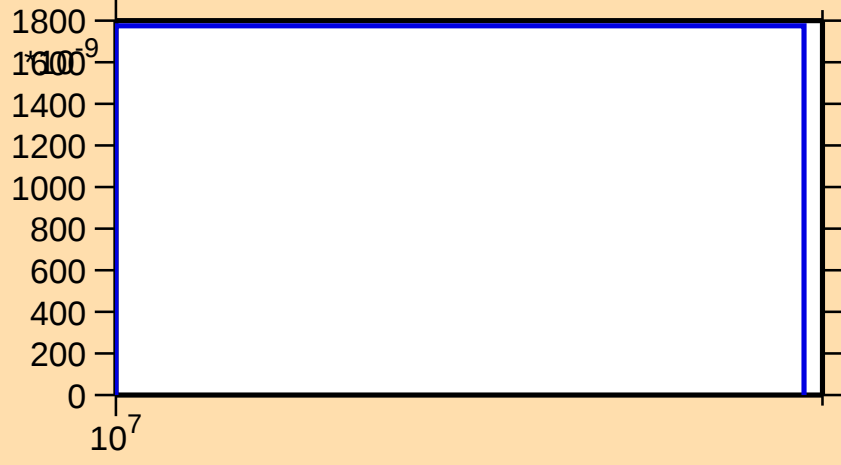
\sigma vs. E for ^{144}\text{Ba}(n,np)
