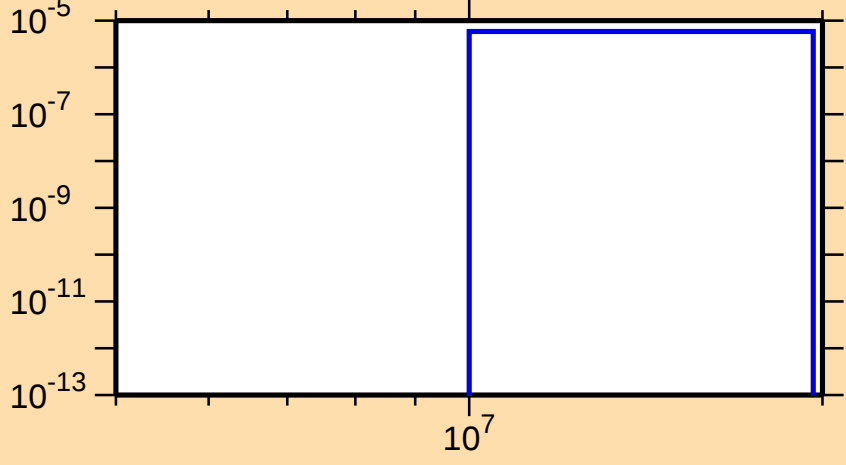
\sigma vs. E for ^{144}\text{Ba}(n,d)
