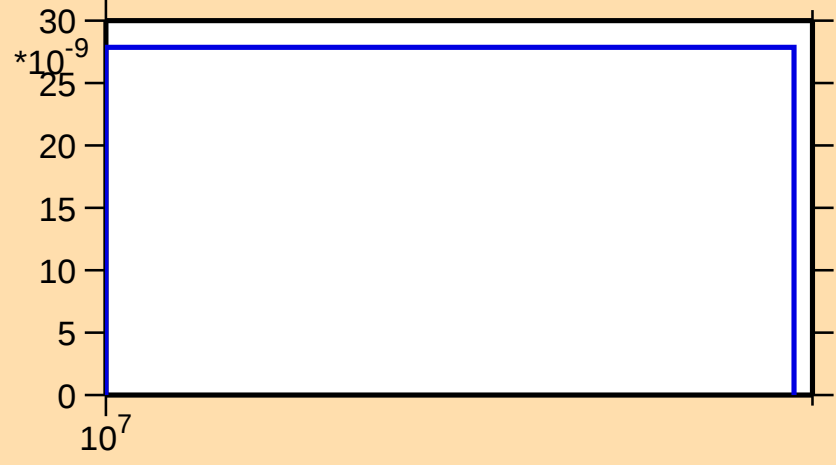
\sigma vs. E for ^{144}\text{Ba}(n,\text{nt})
